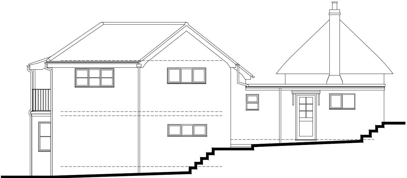
Existing Southeast Elevation Scale - 1:100
