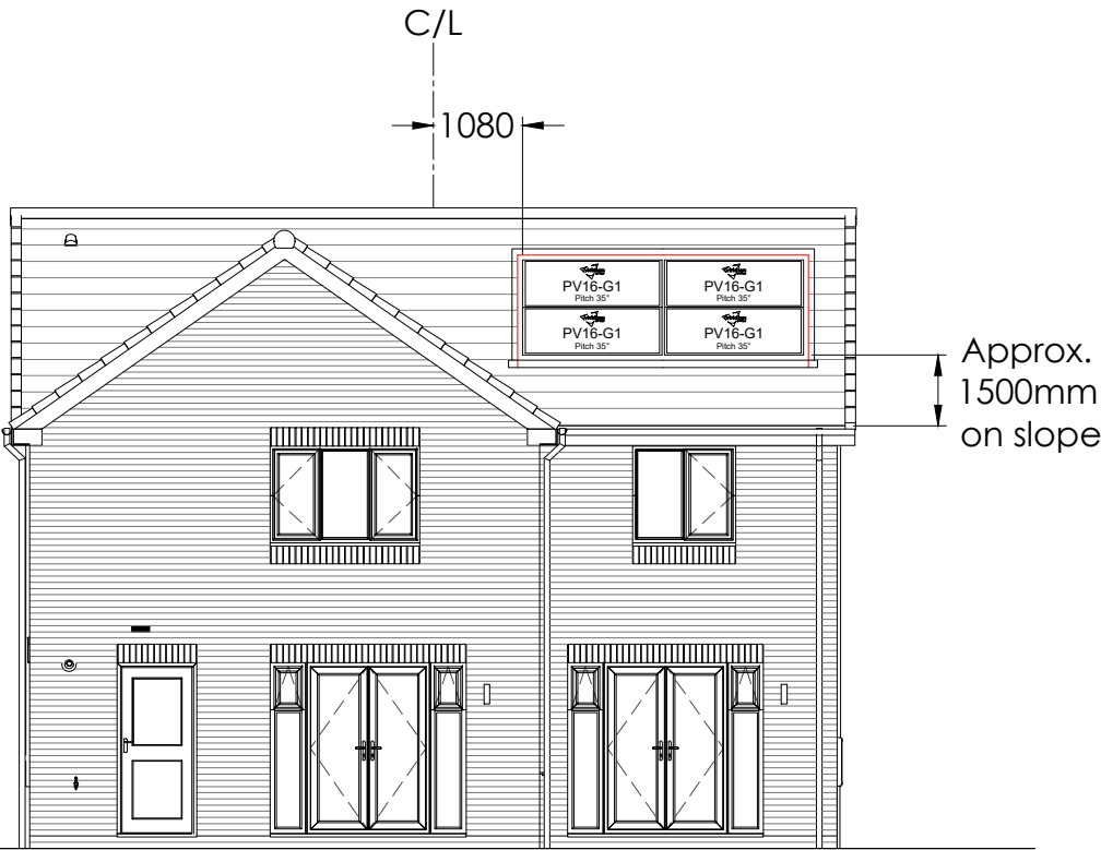
Rear Elevation
