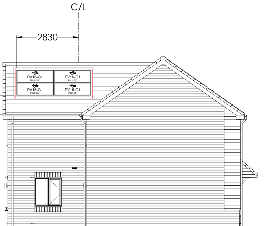
Side Elevation
