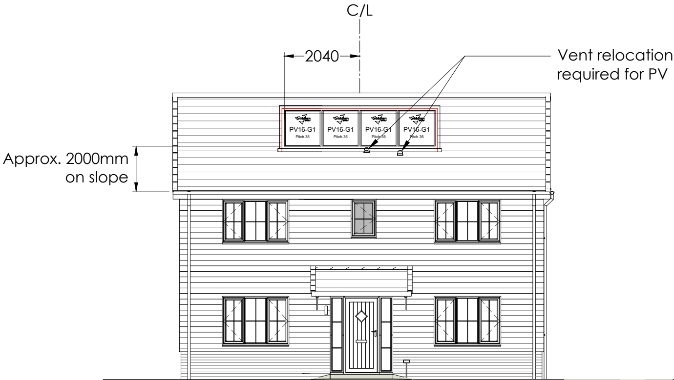
Front Elevation
