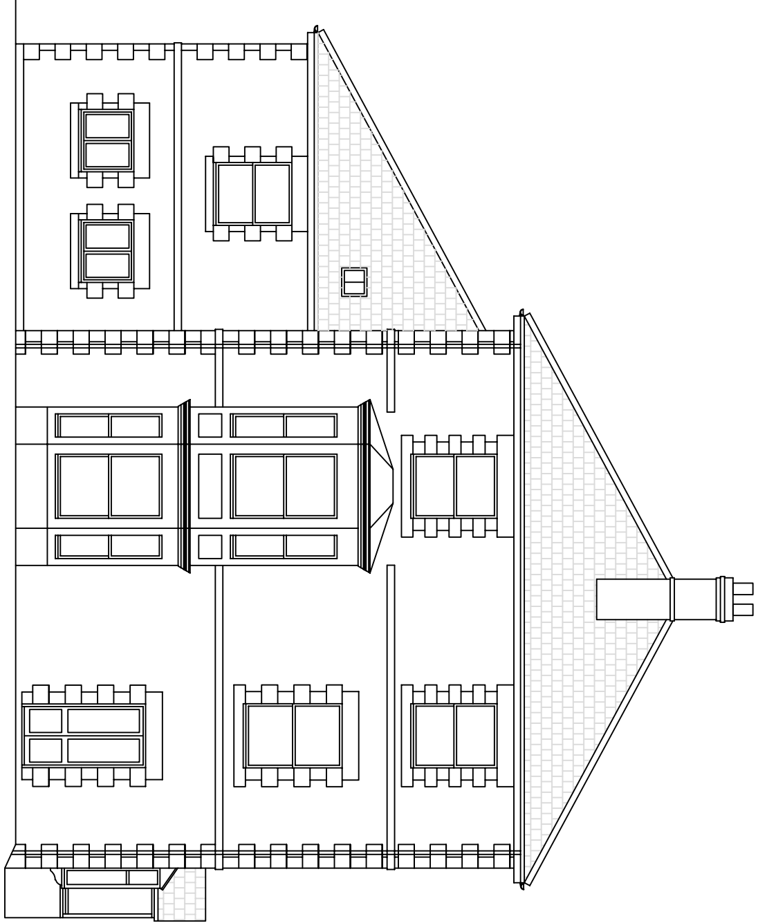
Existing Rear (South) Elevation 1:100
