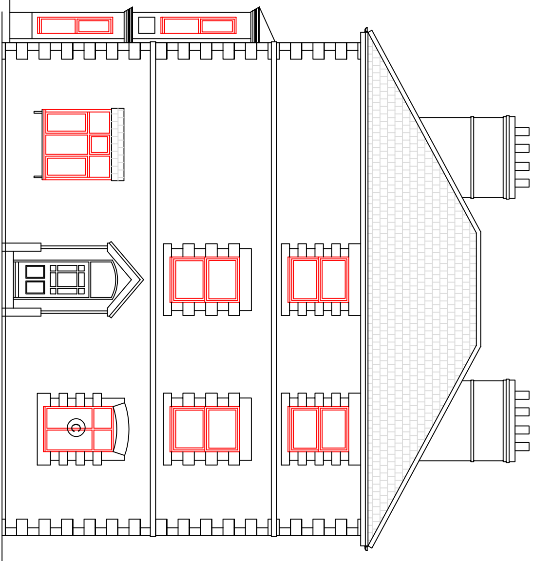
Proposed Side (East) Elevation 1:100
