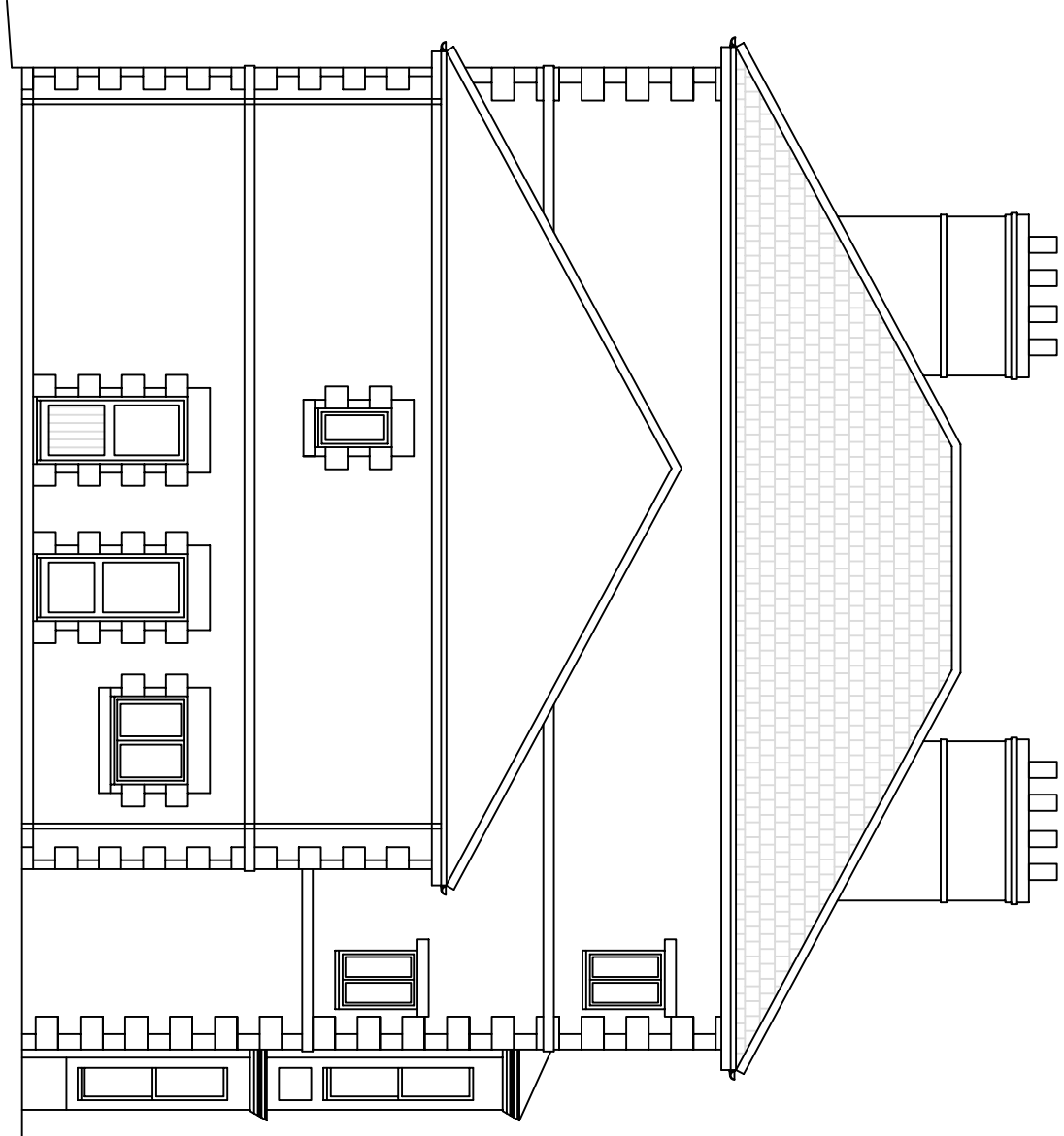
Existing Side (West) Elevation 1:100
