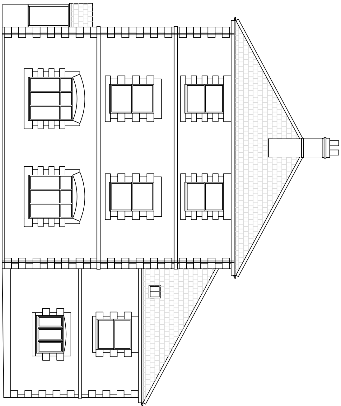
Existing Front (North) Elevation 1:100
