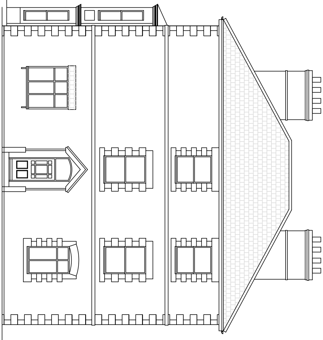
Existing Side (East) Elevation 1:100
