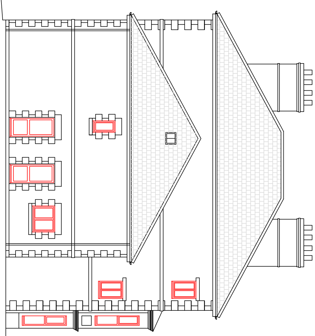
Proposed Side (West) Elevation 1:100
