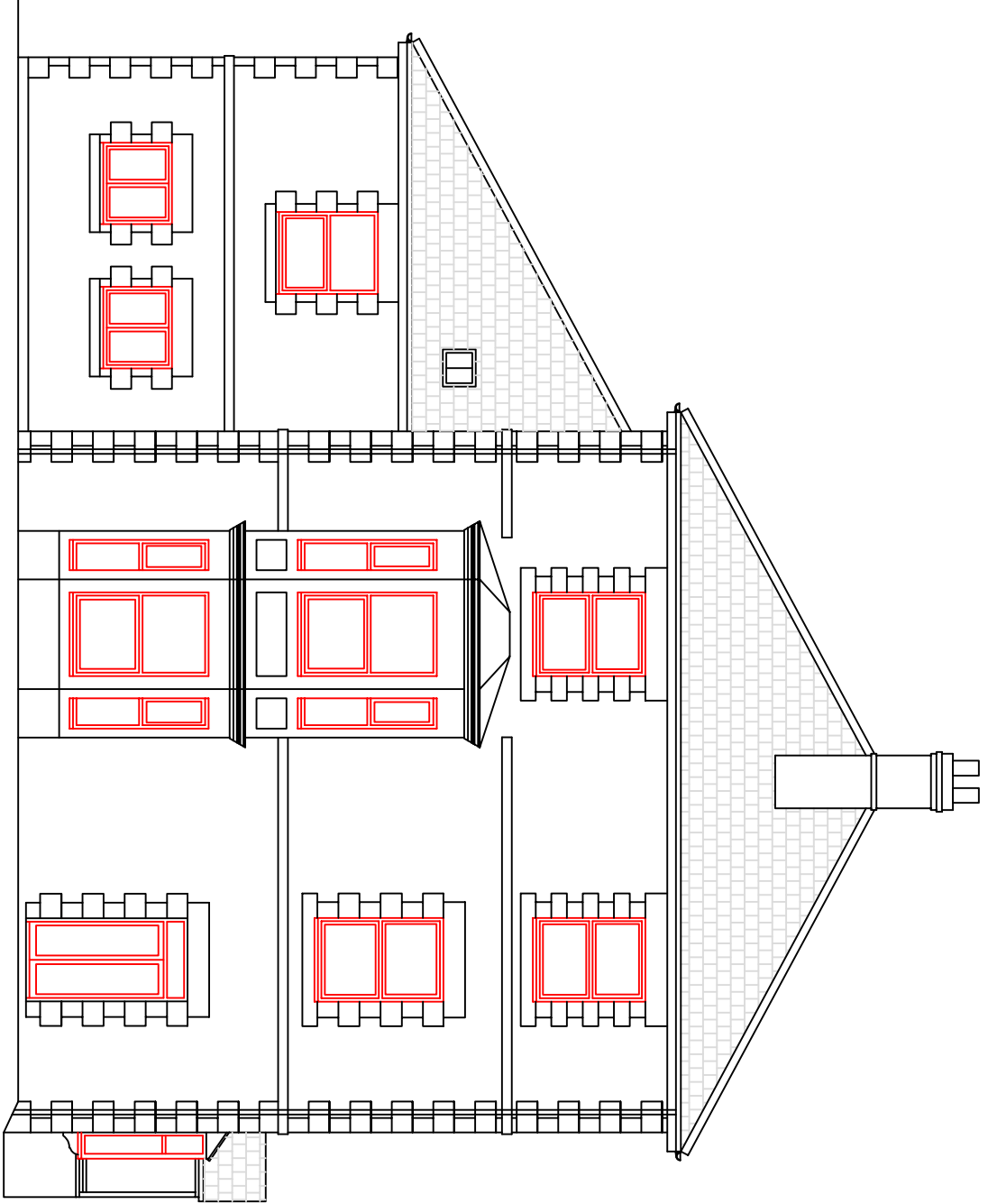
Proposed Rear (South) Elevation 1:100
