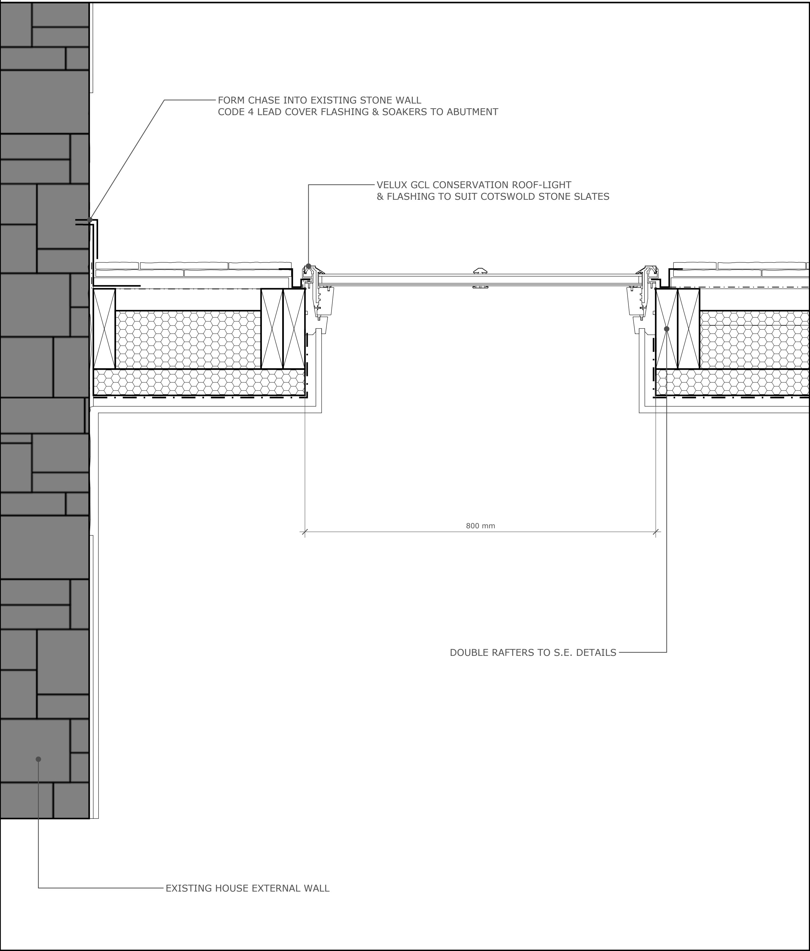
ABUTMENT DETAIL 1
