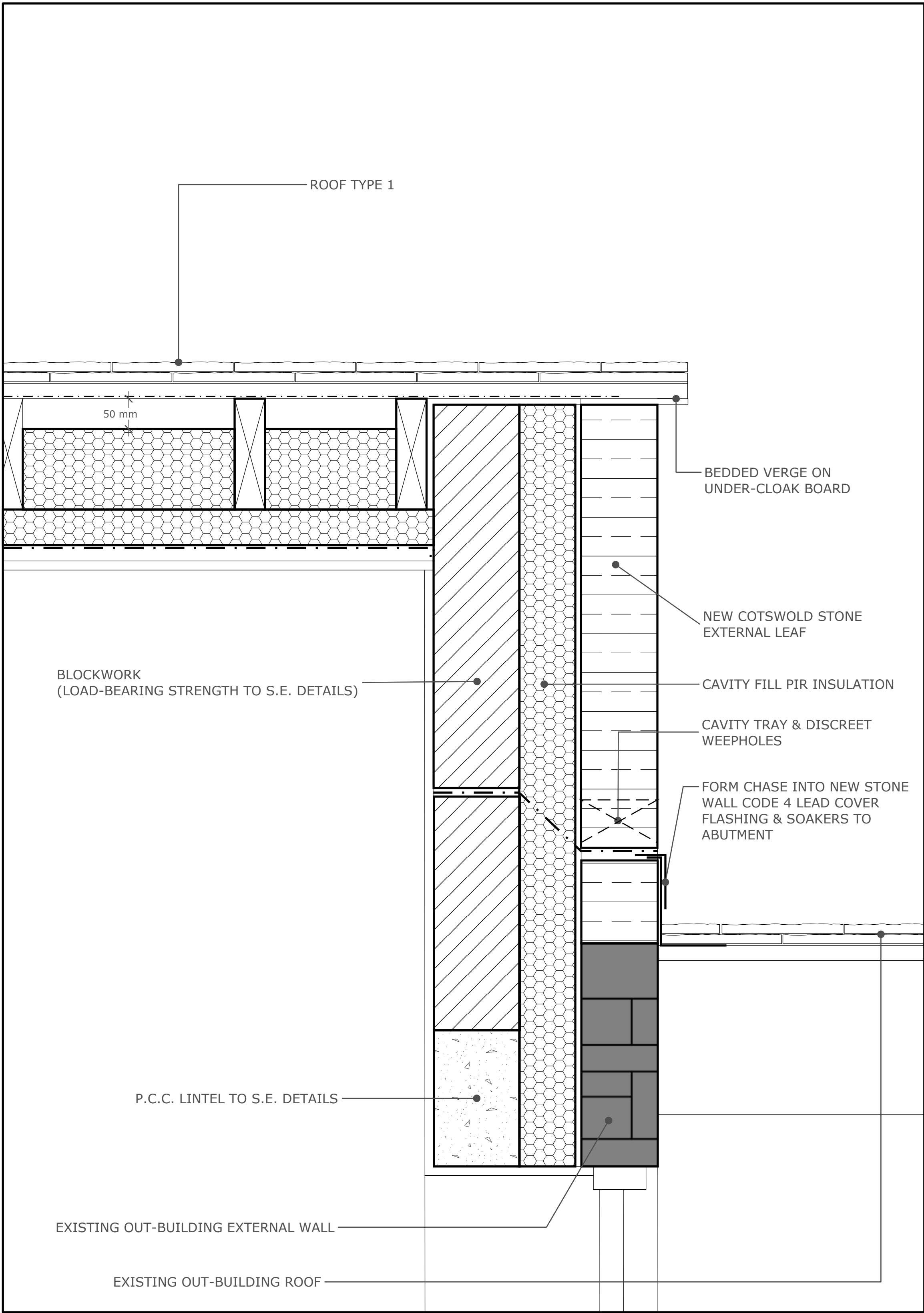
VERGE DETAIL 1
