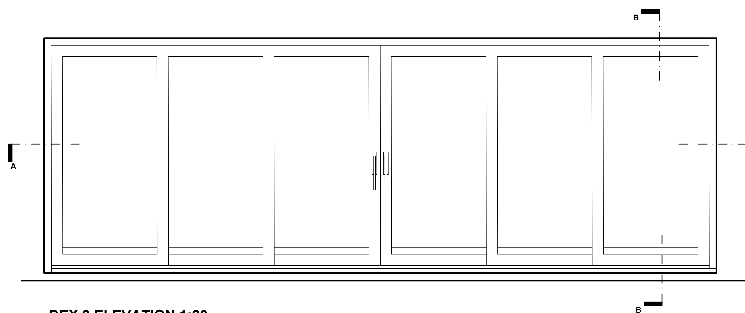
DEX 3 ELEVATION 1:20
