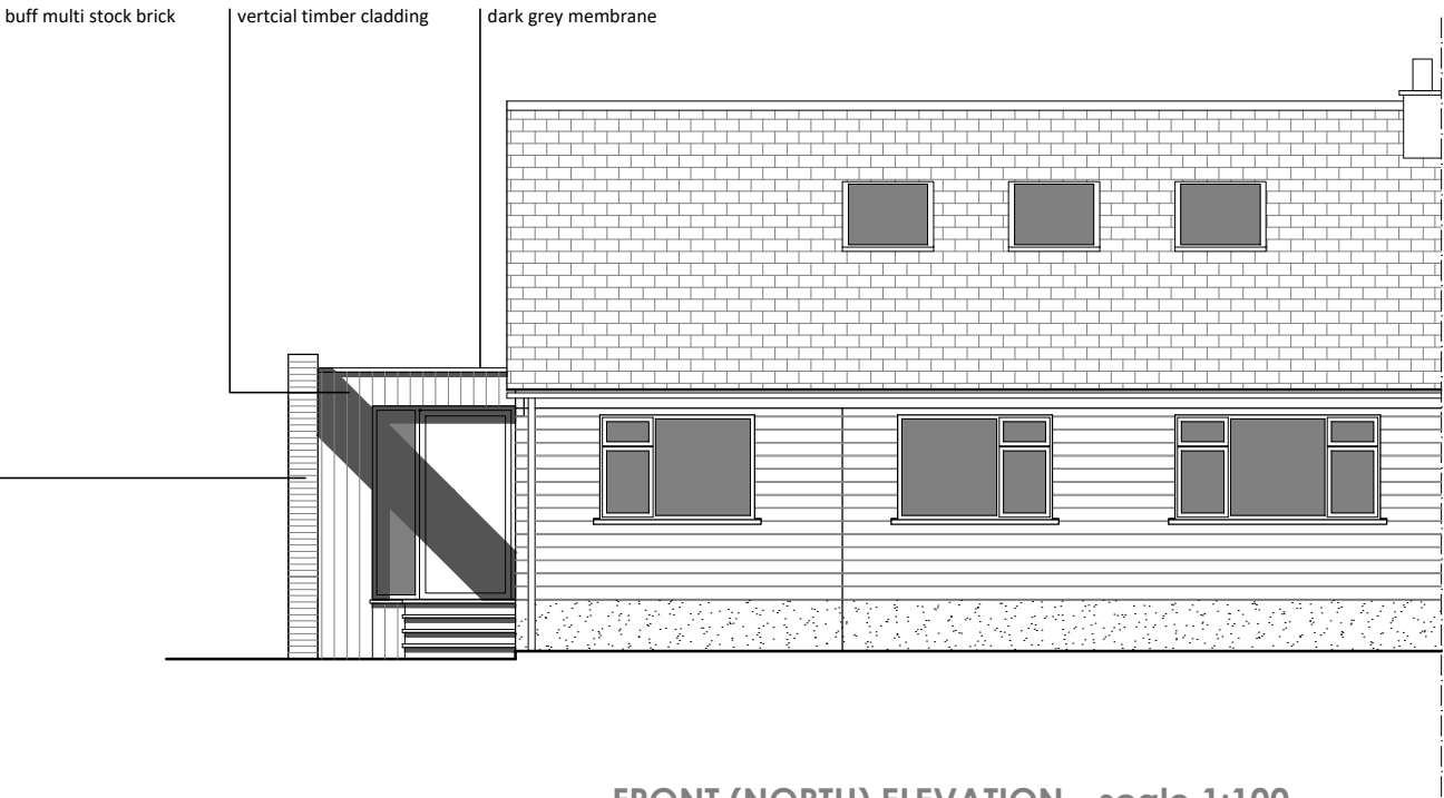
FRONT (NORTH) ELEVATION - scale 1:100
