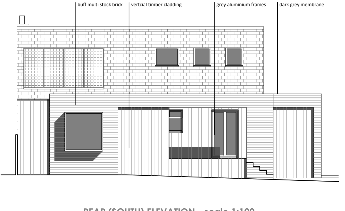
REAR (SOUTH) ELEVATION - scale 1:100
