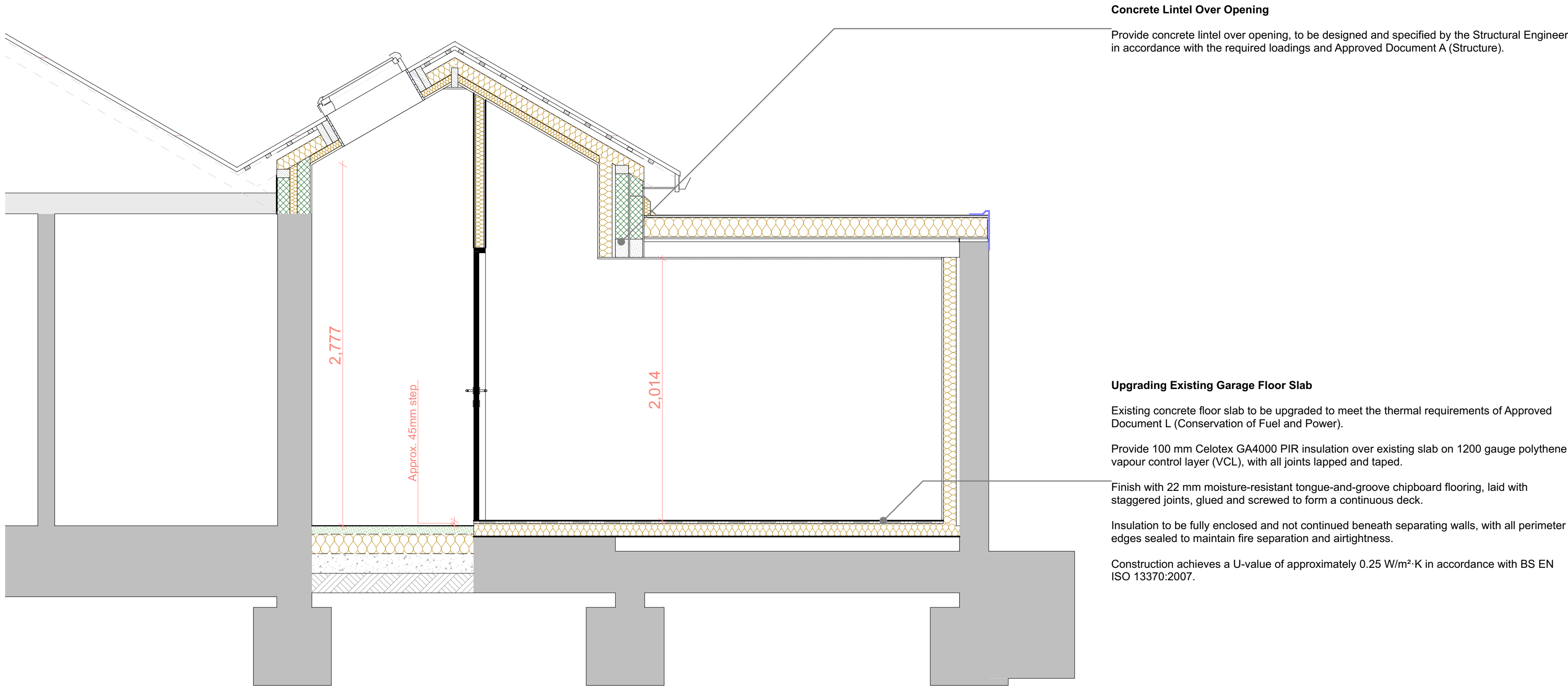
SECTION B-B
