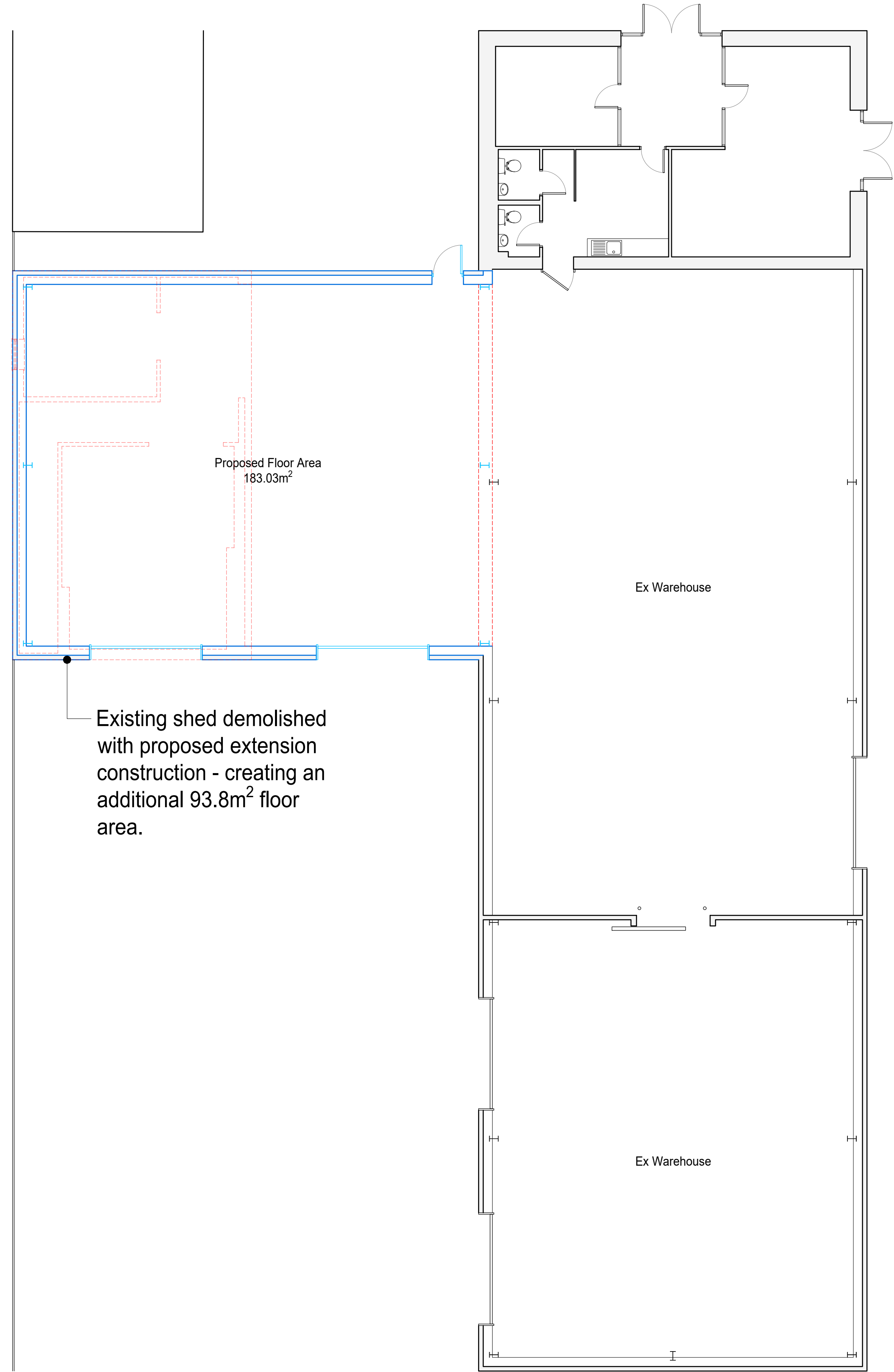
Proposed Floor Plan - 1:100
