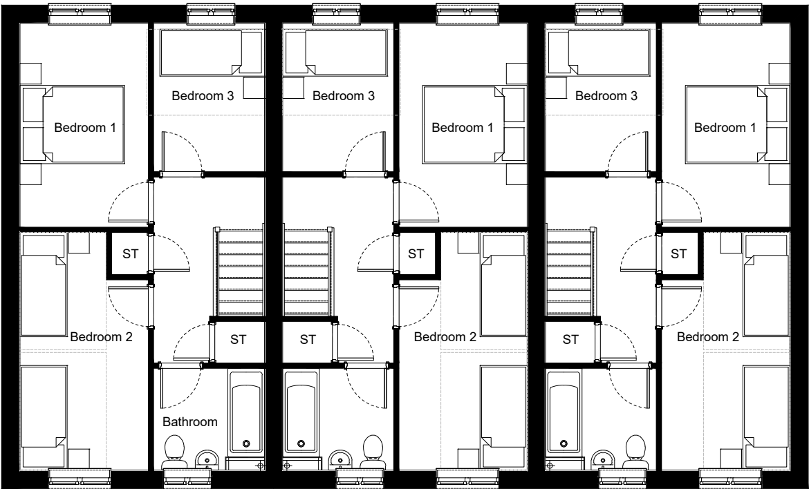
House Type A3 - First Floor Plan
