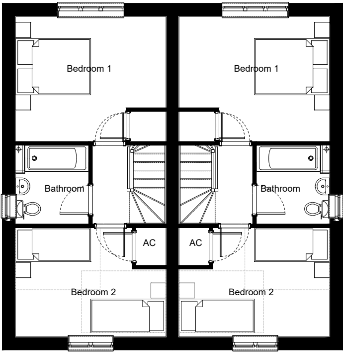
House Type A2 - First Floor Plan
