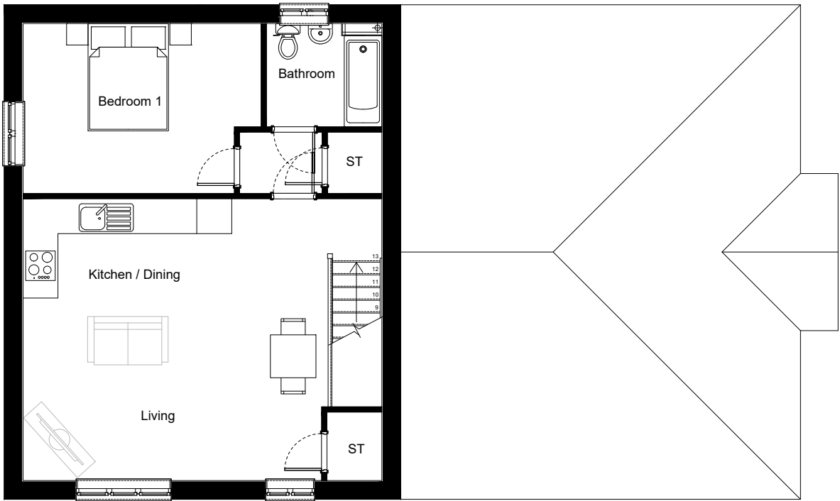
House Type A1M First Floor Plan
