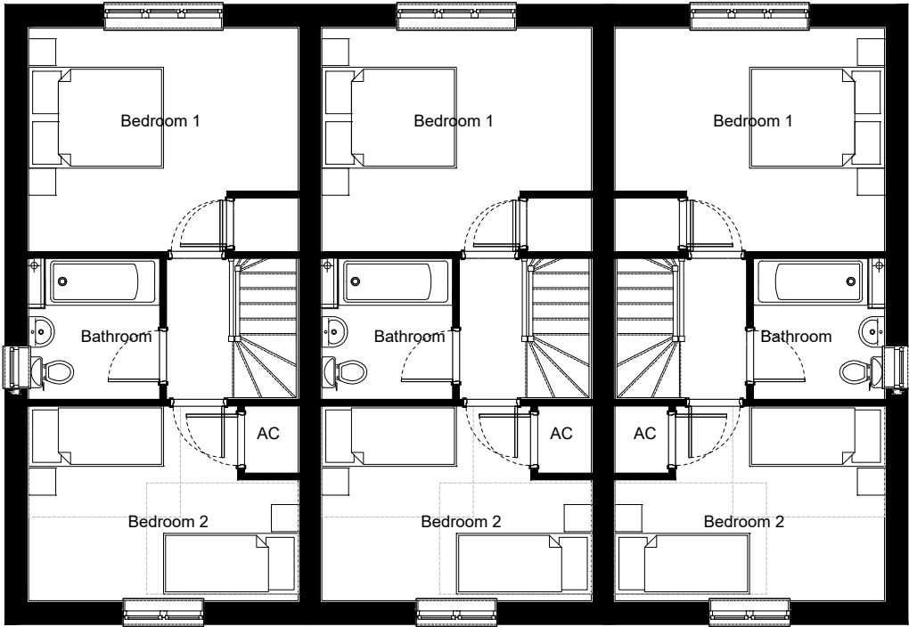
House Type A2 - First Floor Plan
