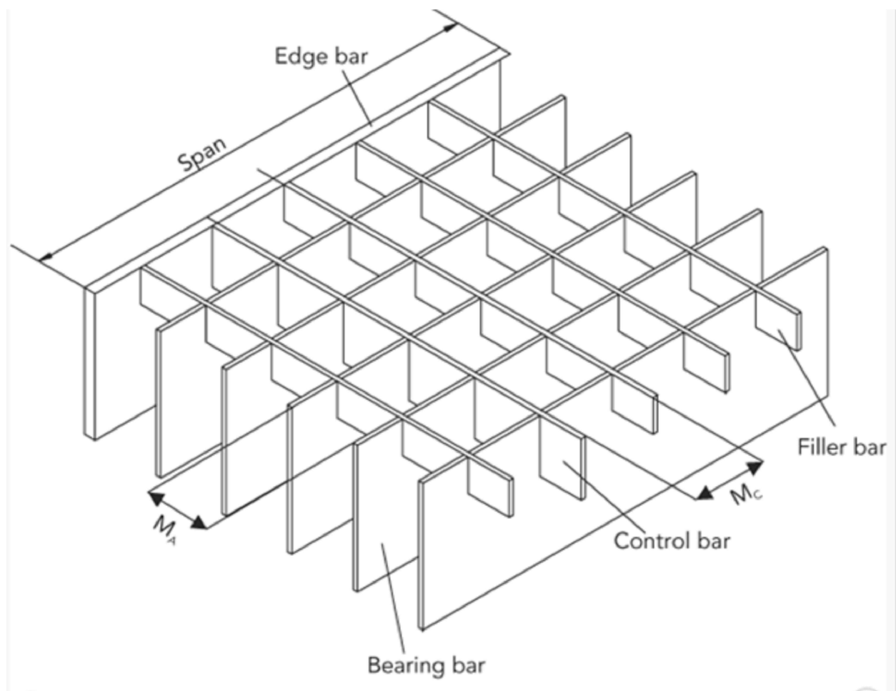
PROPOSED HEEL GUARD METAL GRATING DIAGRAM (NOT TO SCALE)
