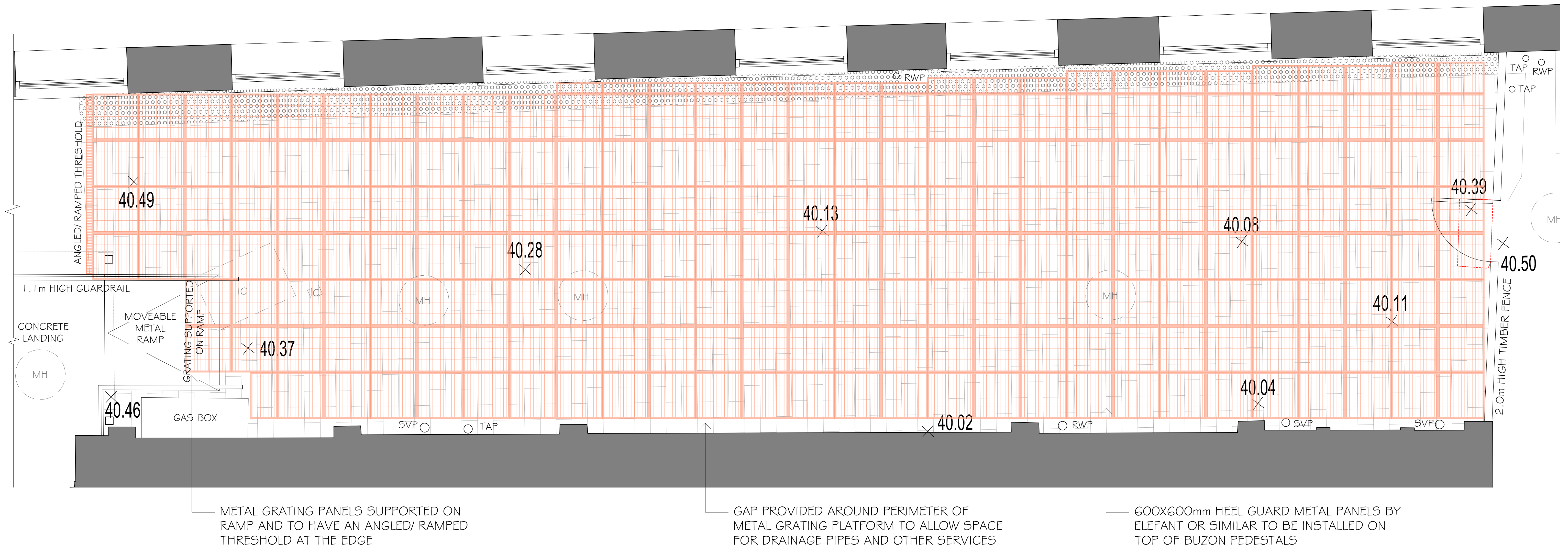
PROPOSED COURTYARD LAYOUT - METAL GRATING LAYOUT scale 1:25
