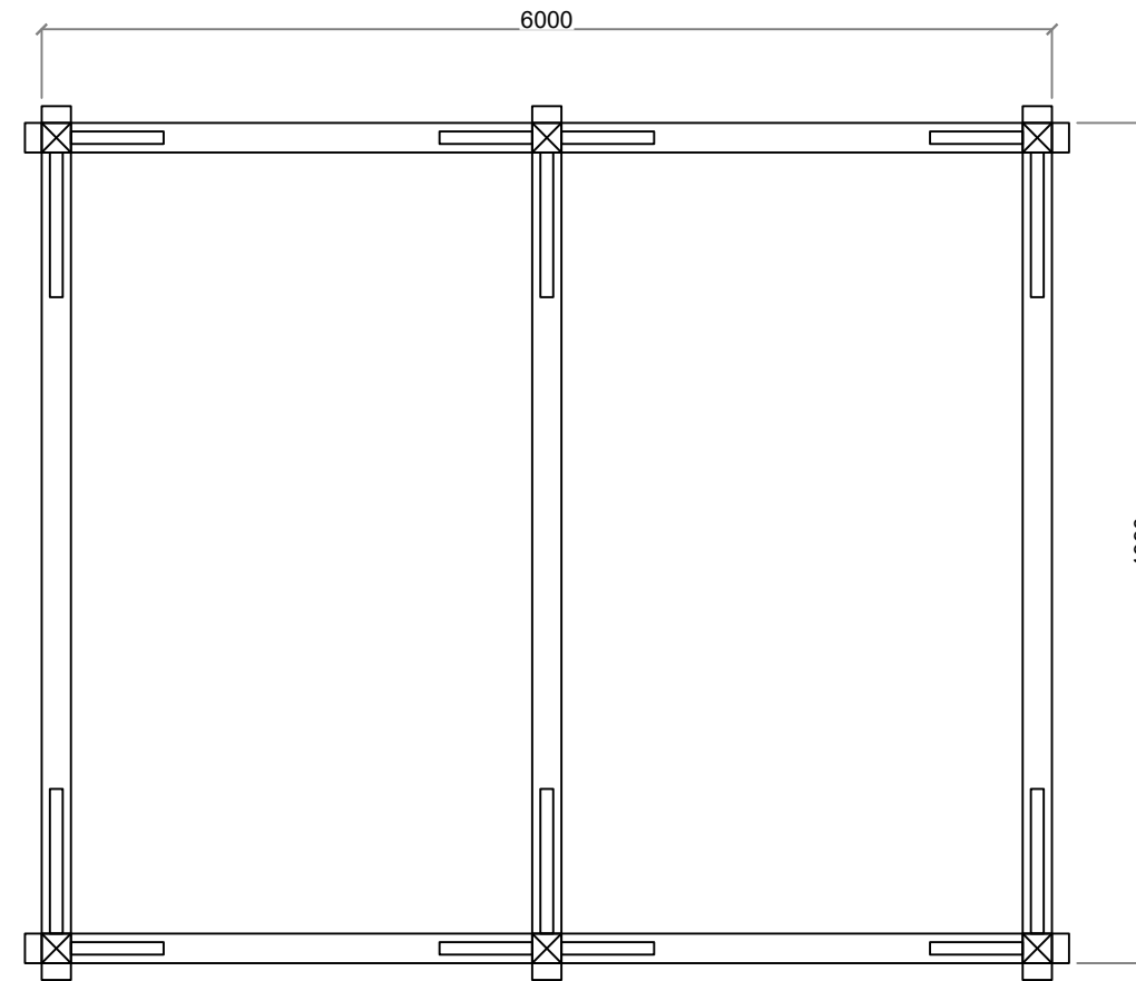
Floor / Frame Plan
