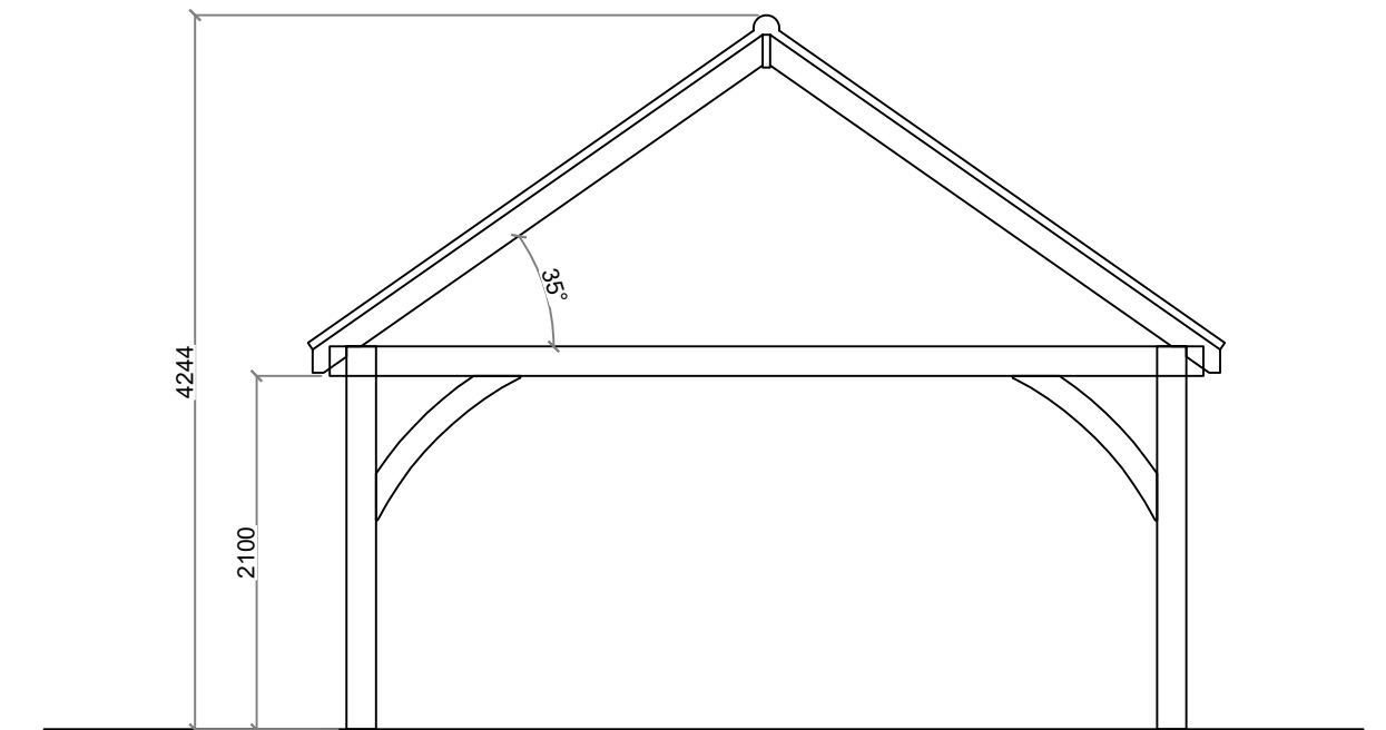
Section
