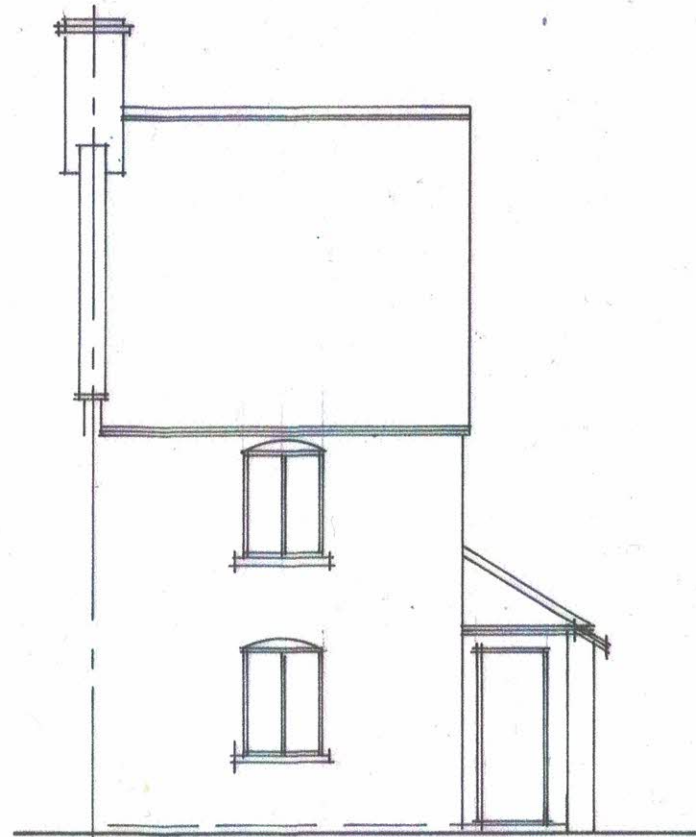
WEST
