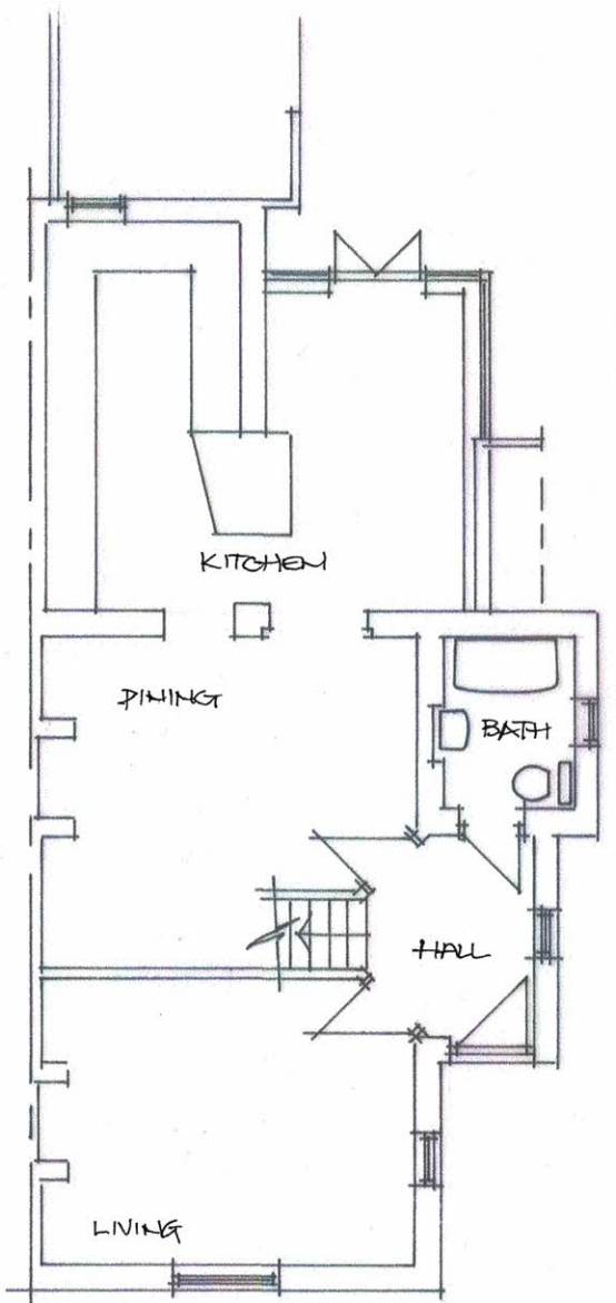
GROUND
