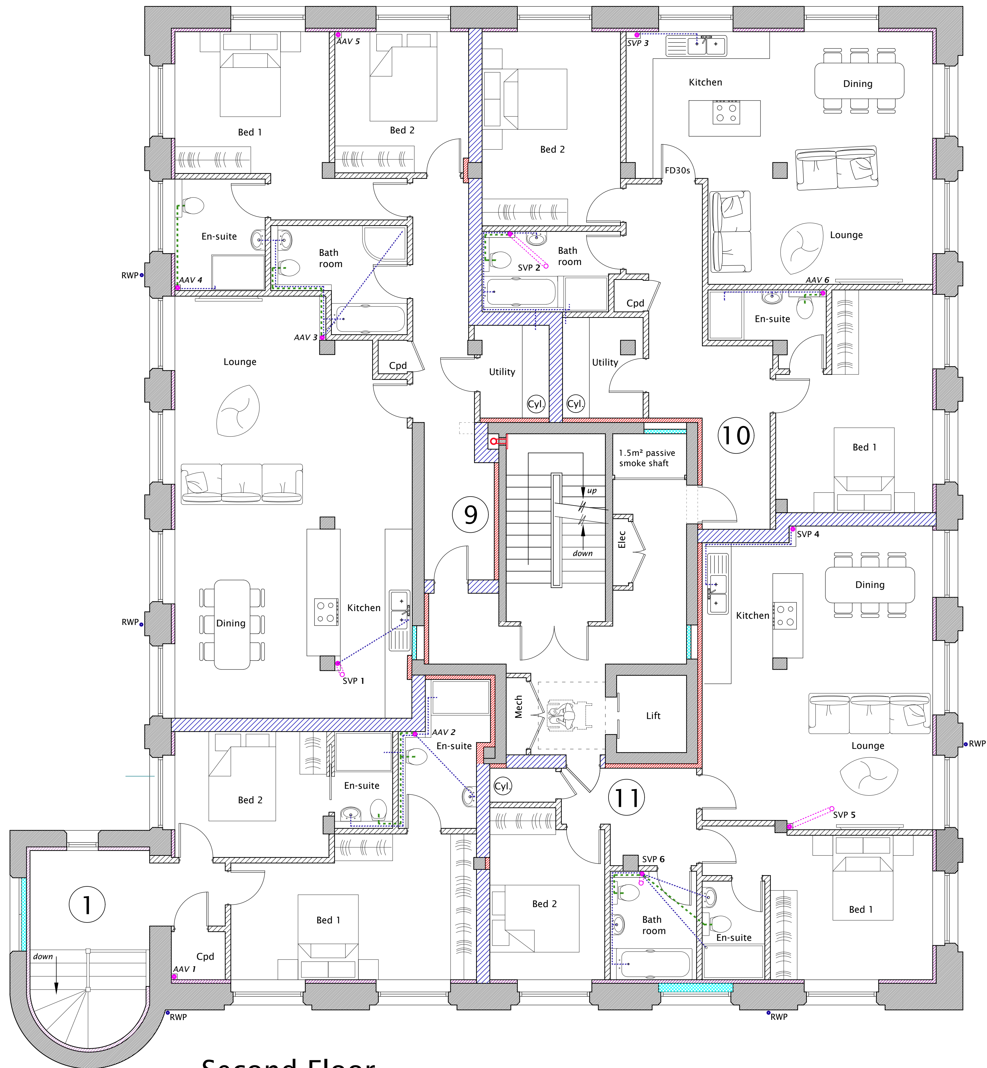
Second Floor scale 1:50
