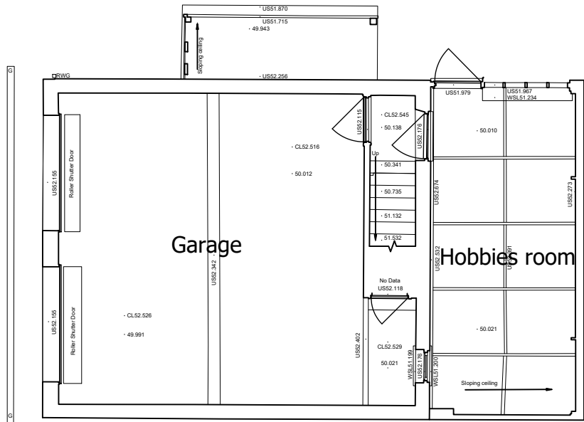
ANNEXE GROUND FLOOR PLAN
