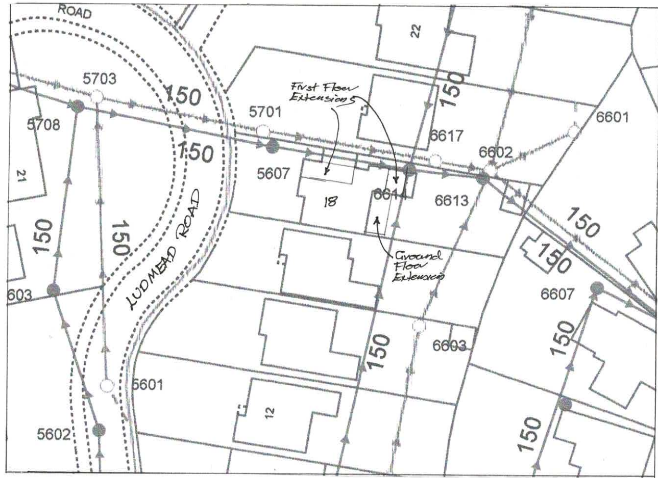
Block Plan 1:500
