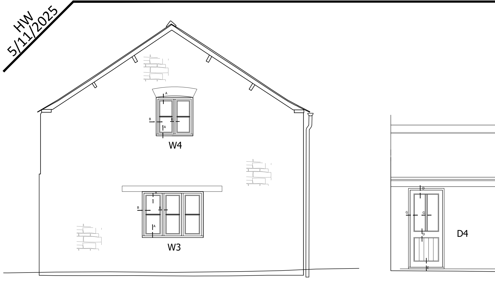
West elevation
