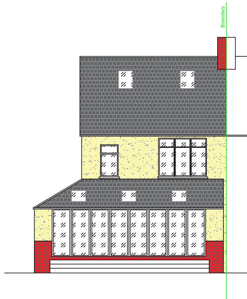
REAR (NORTH) ELEVATION - PROPOSED
