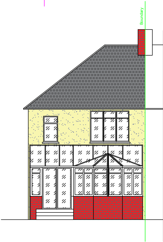
REAR (NORTH) ELEVATION - EXISTING
