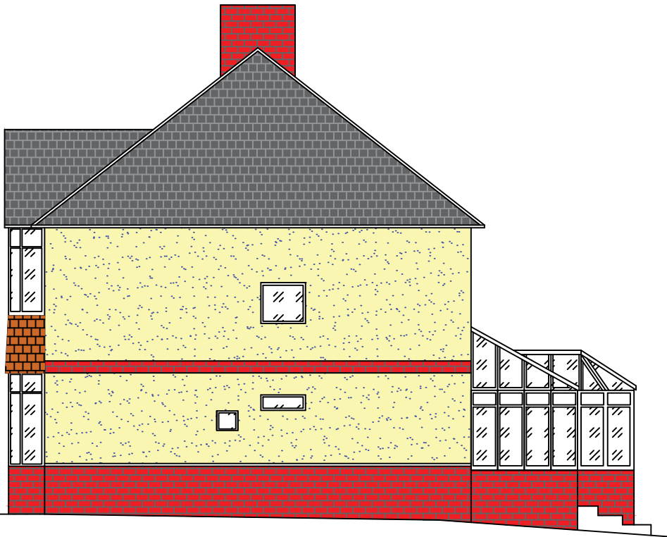
SIDE (EAST) ELEVATION - EXISTING
