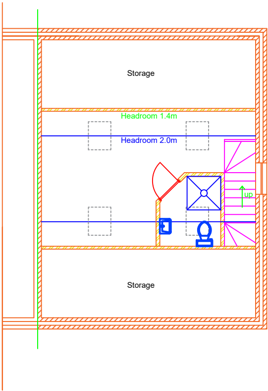
LOFT PLAN - PROPOSED
