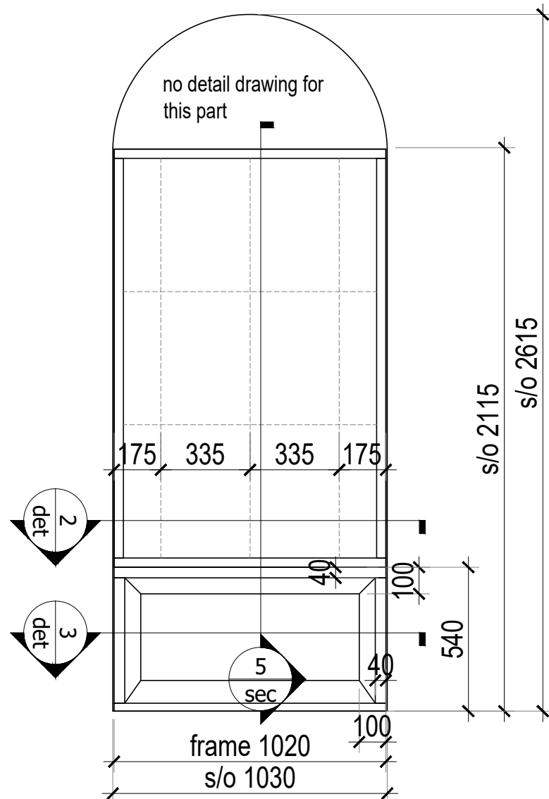
1. Elevation 1:20
