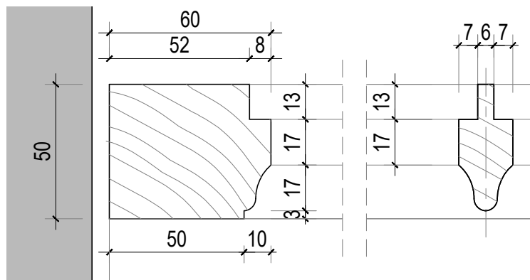
3. Detail
