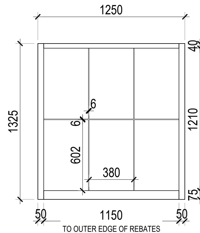
9. Bottom Sash - elevation
