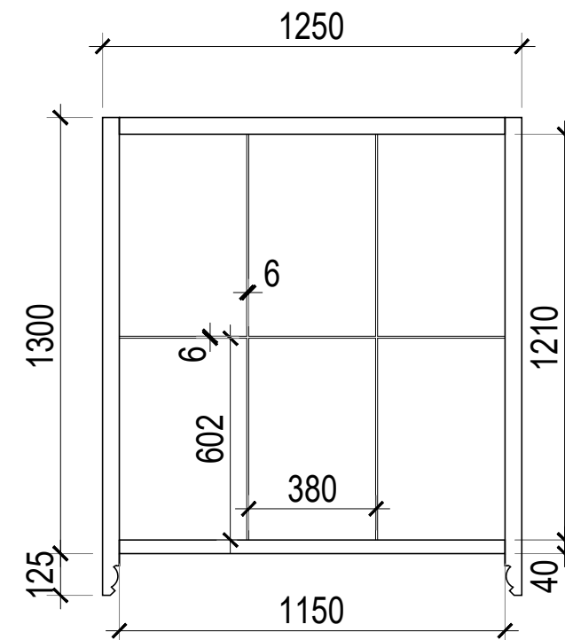
8. Top Sash - elevation
