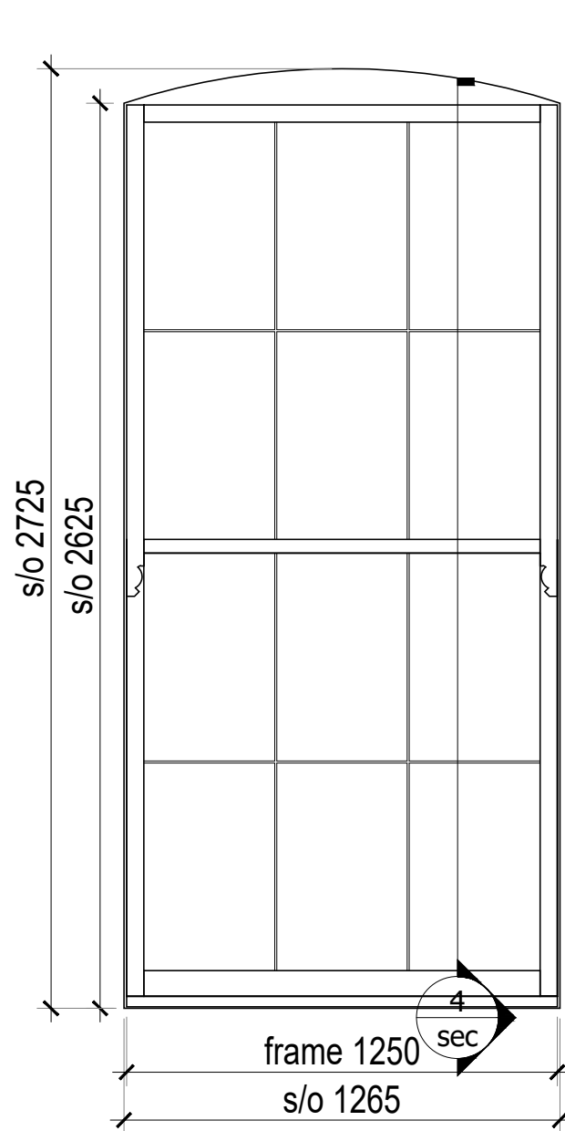
1. Elevation 1:20
