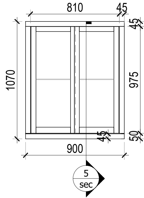
1. Elevation 1:20
