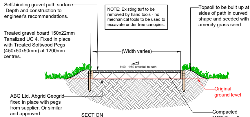
SECTION NO-DIG SELF BINDING GRAVEL PATH ADJACENT TO TREE ROOTS
