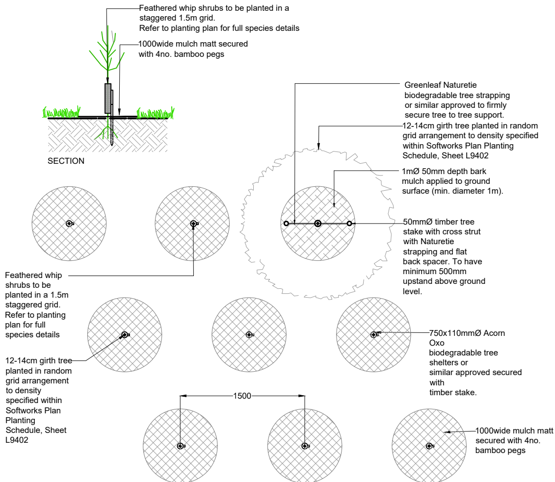
PLAN SCRUB WITH EMERGENT WOODLAND PLANTING
