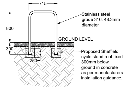
SECTION CYCLE HOOPS - 2NO. SHEFFIELD CYCLE STANDS (OR SIMILAR AND APPROVED)
