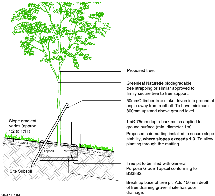
SECTION TYPICAL TREE PIT DETAIL TO BANKED AREA
