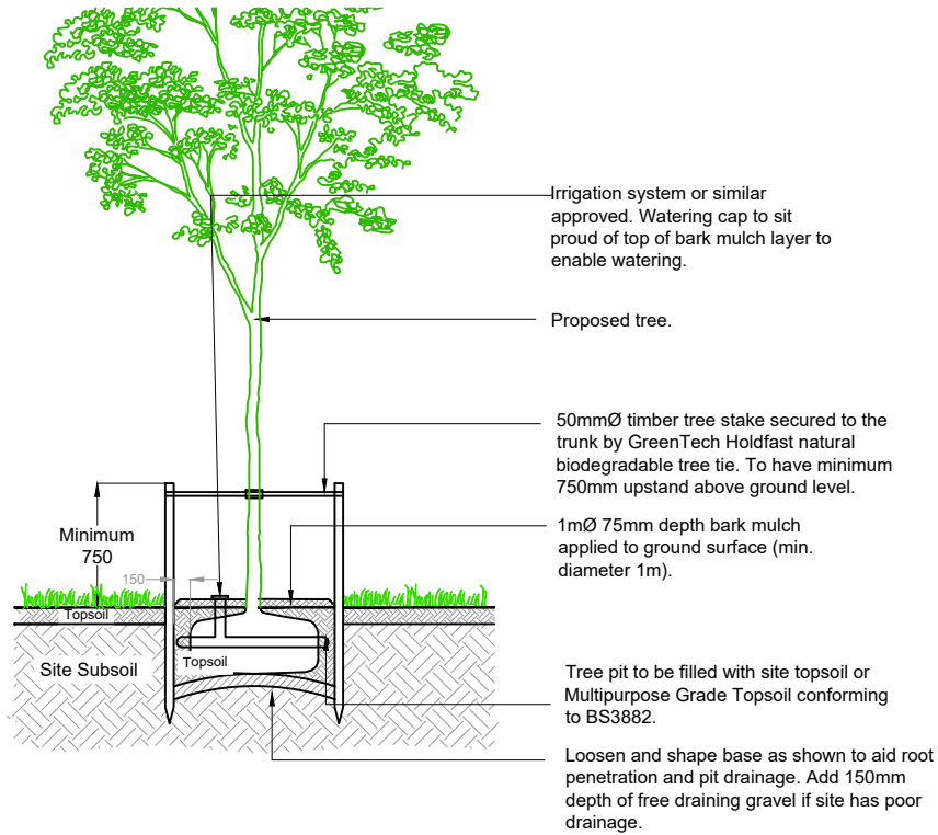
SECTION PROPOSED TREE PLANTING TO BE DOUBLE STAKED
