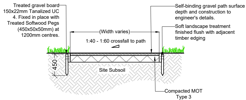
SECTION SELF BINDING GRAVEL PATH
