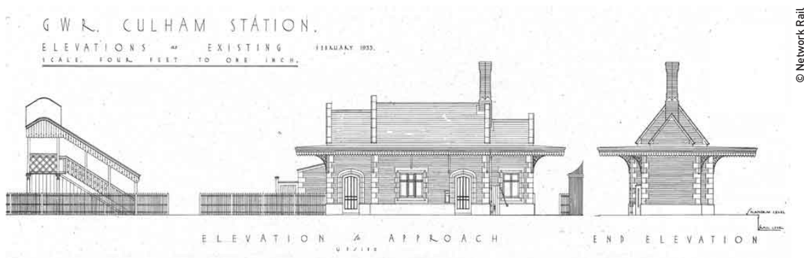
Fig. 18: Brunel's 1844 Culham Station 'chalet' structure drawn as it existed in 1935 and showing daggerboard valancing to the canopy
