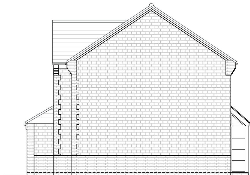
PROPOSED NORTH EAST ELEVATION
