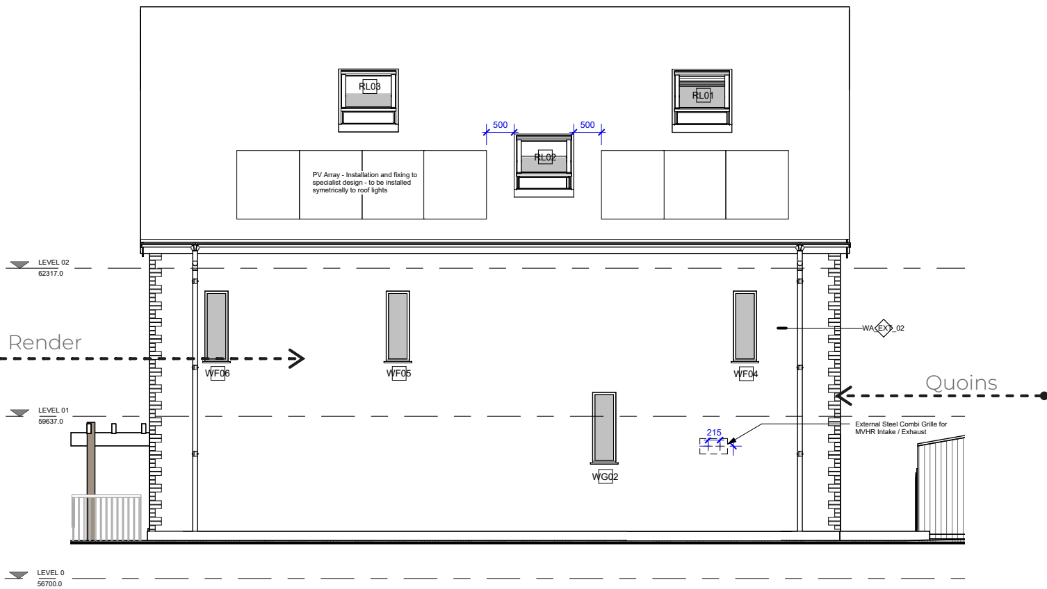
Fig.3 Proposed North and East Elevation Finishes (East Elevation shown above)
