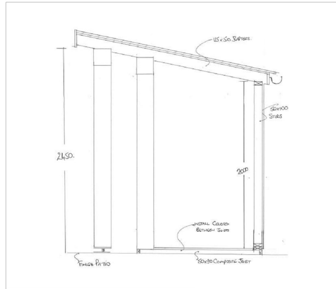
Original Construction Drawing of Outdoor Kitchen Outbuilding - NTS
