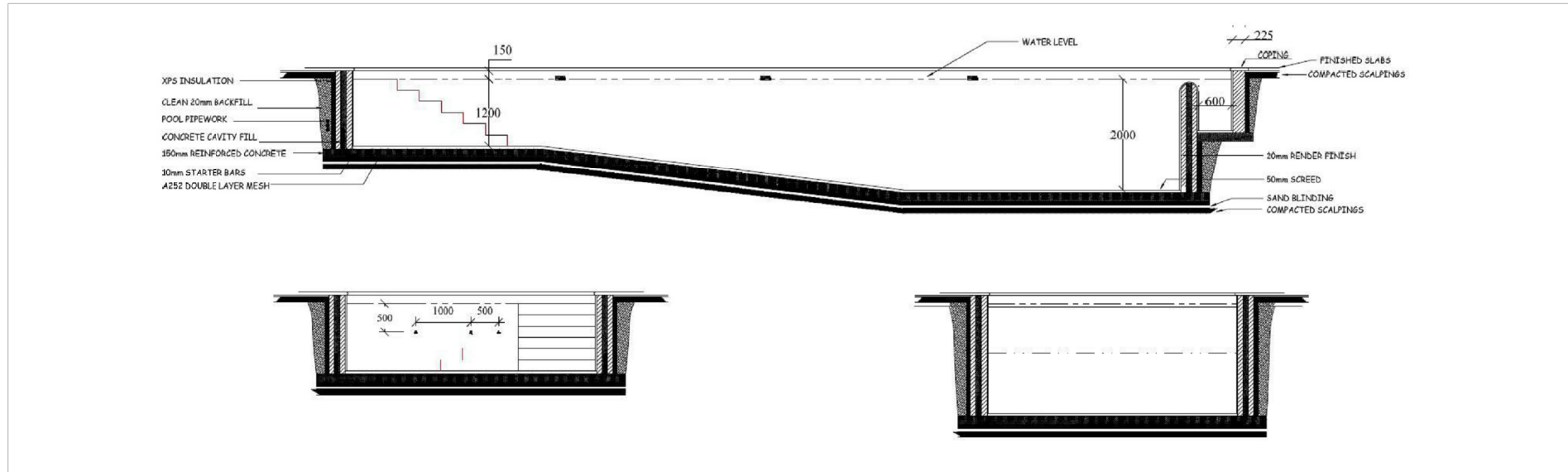
Original Construction Drawings of New Swimming Pool - NTS
