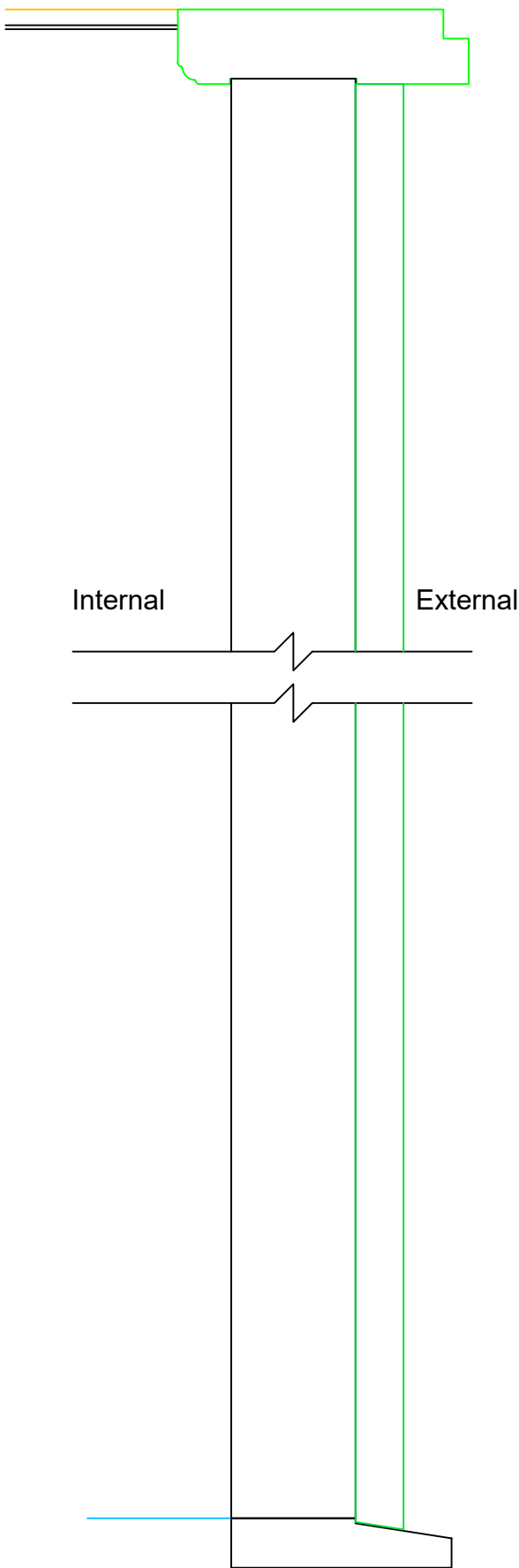
VERTICAL VIEW THROUGH FULL HEIGHT PILASTER
