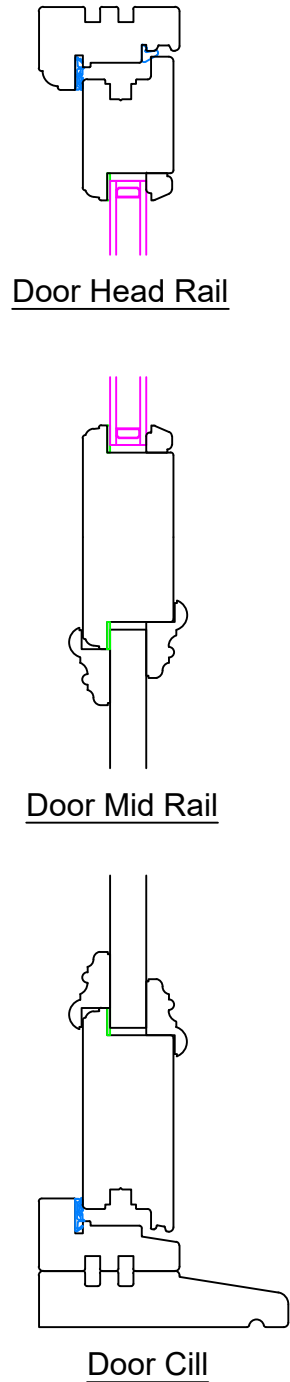
VERTICAL VIEW THROUGH DOUBLE DOOR
