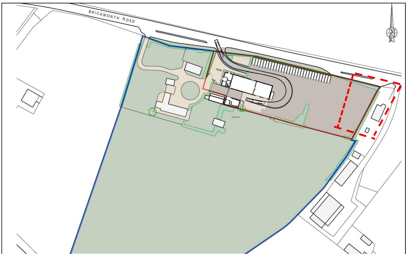
Figure 1 Site layout and operation restrictions.
