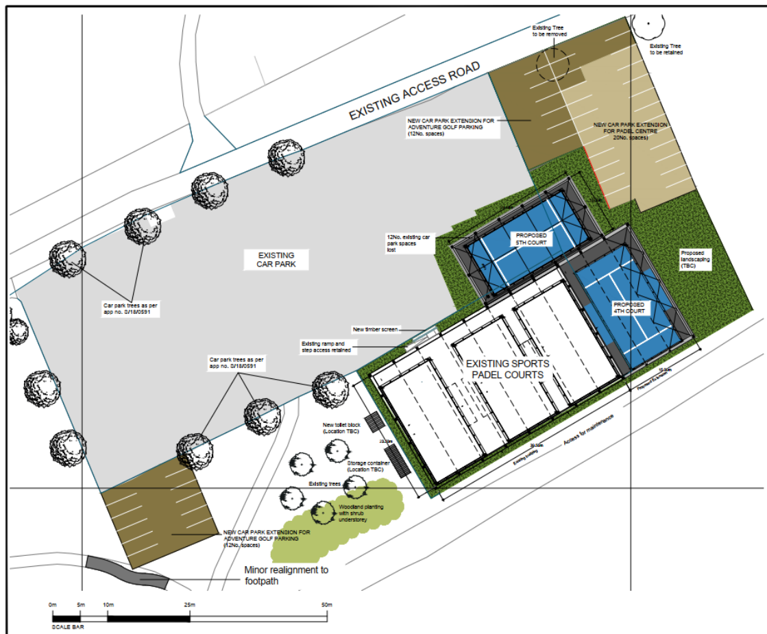
Figure 2: Site Location – Padel Courts
