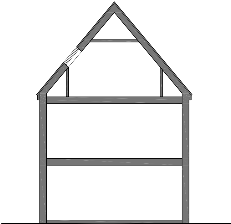
Section (through living room/bed 1)
