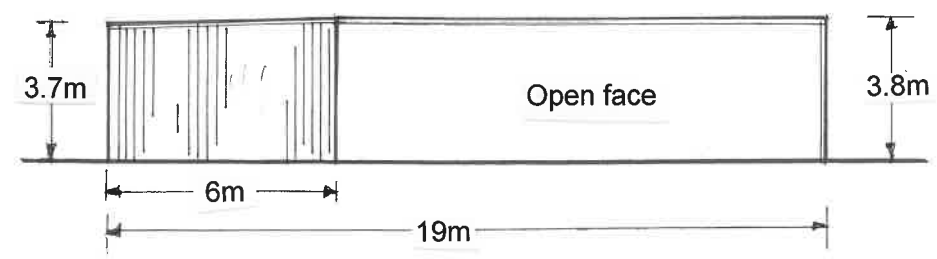
NORTH ELEVATION
