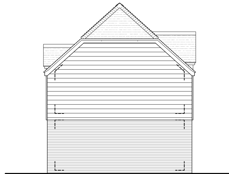
NE ELEVATION Plot 3
