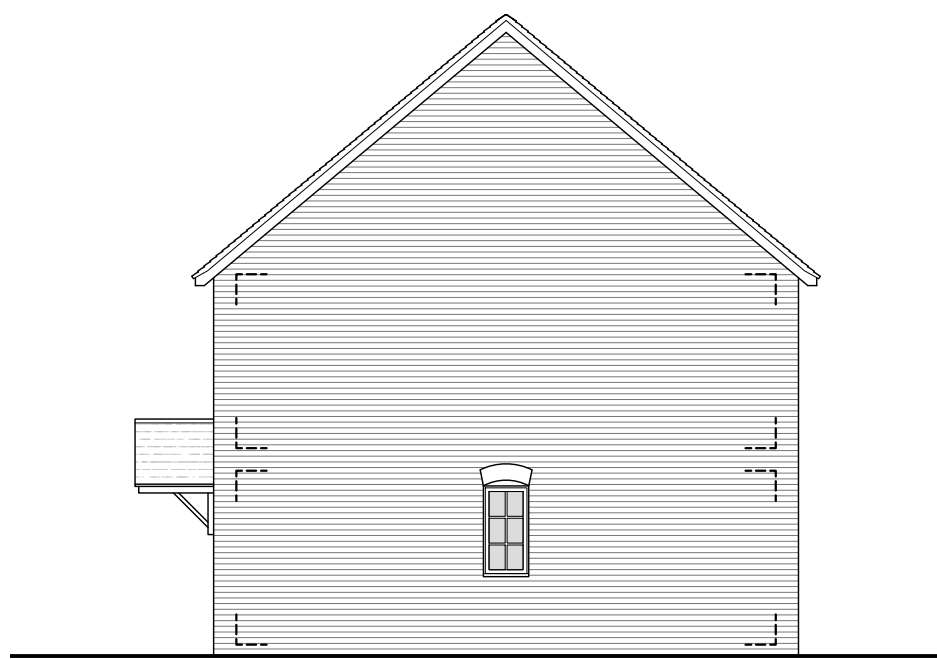
NW ELEVATION Plot 1 & 2
