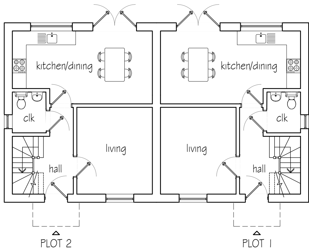
GROUND FLOOR PLAN Plot 1 & 2
