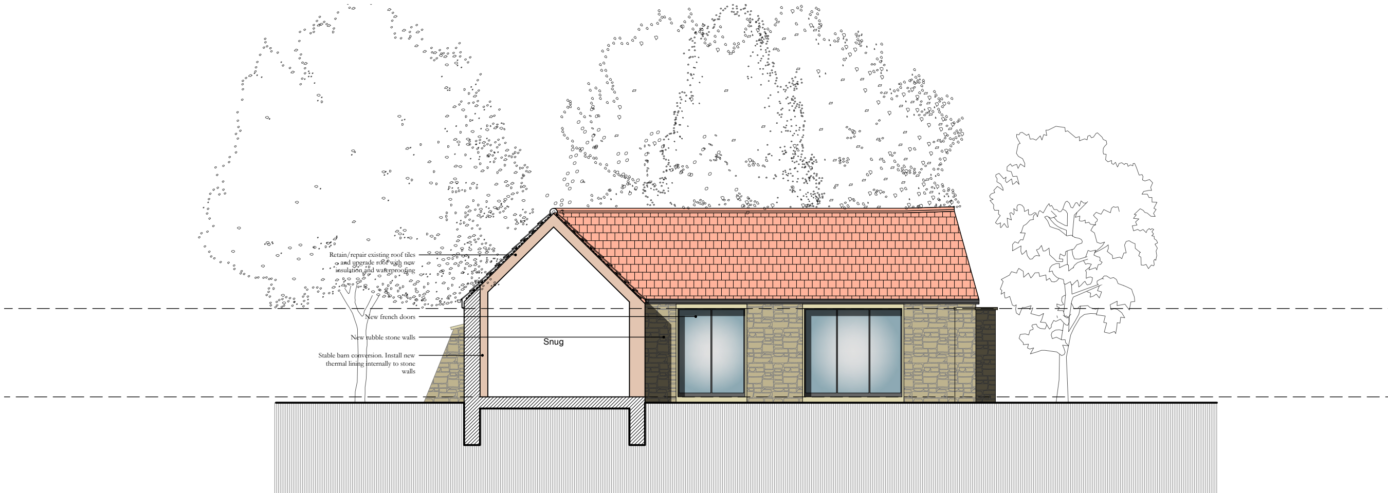
0 5m Section BB Proposed
