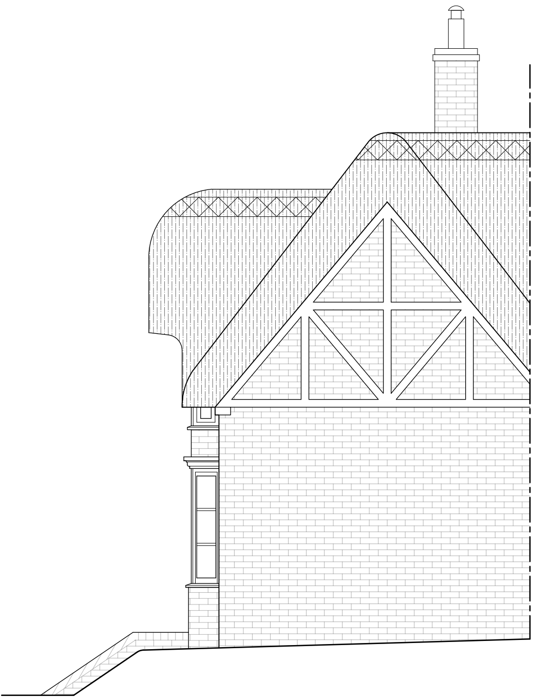
EXISTING PART NORTH ELEVATION Scale 1:50
