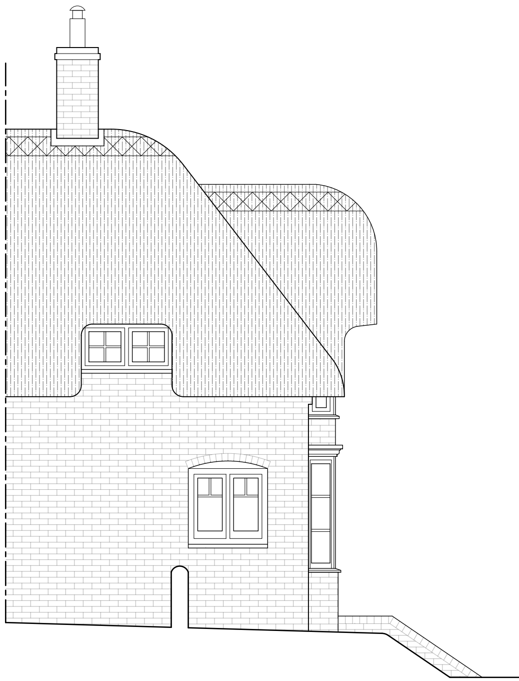
EXISTING PART SOUTH ELEVATION Scale 1:50
