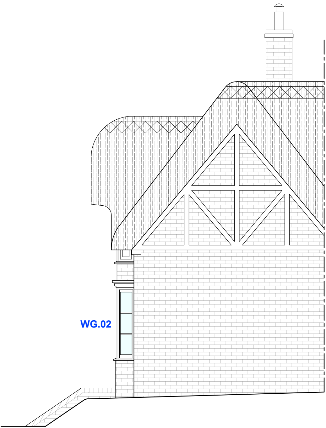
PROPOSED PART NORTH ELEVATION Scale 1:50
