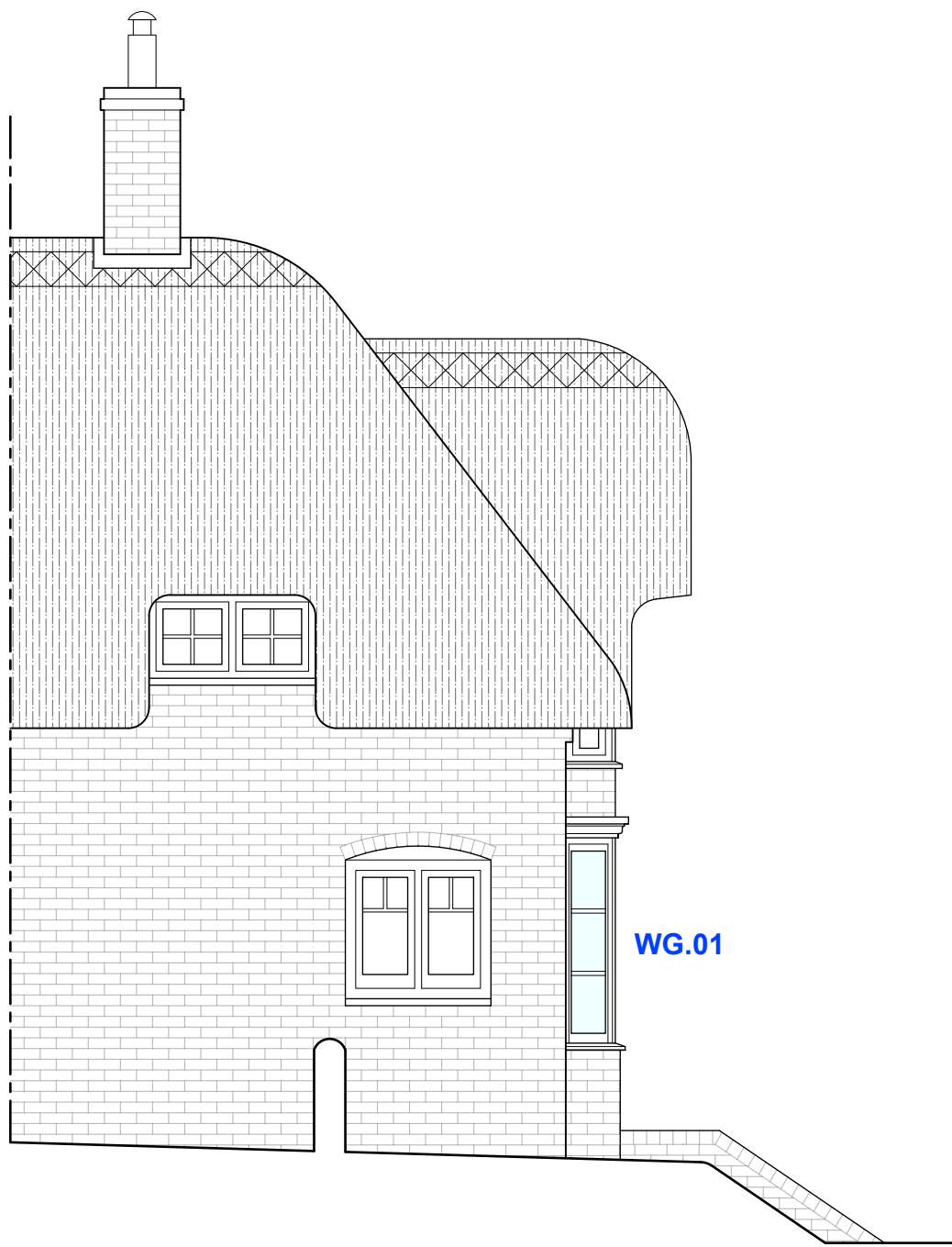
PROPOSED PART SOUTH ELEVATION Scale 1:50
