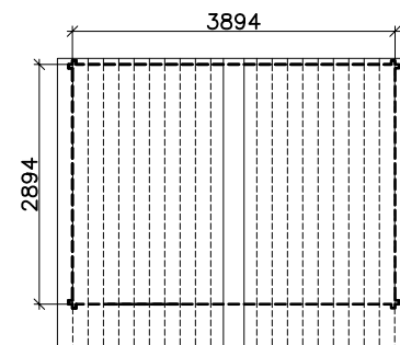
Roof Plan
