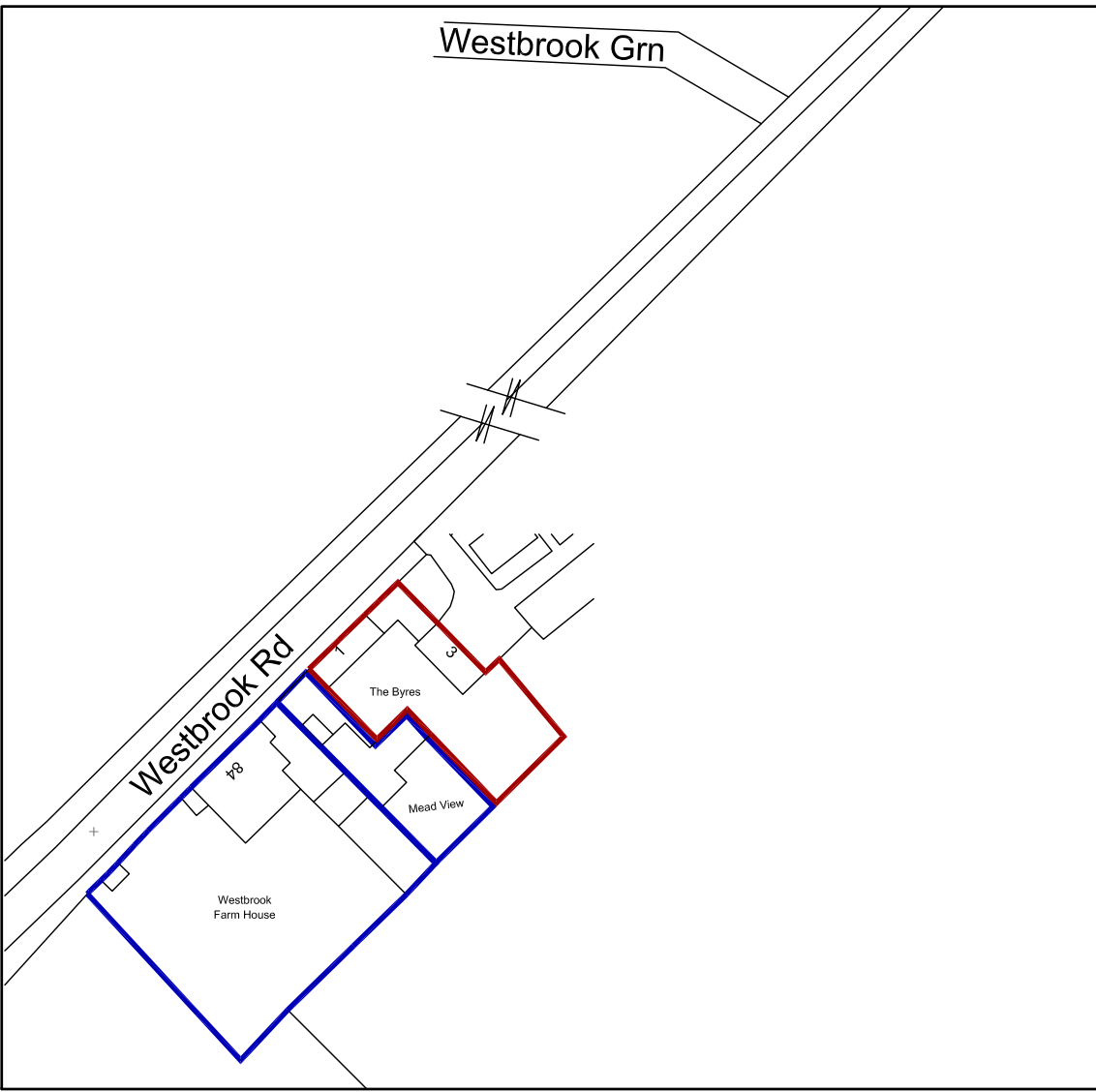
Location Plan 1:1250
