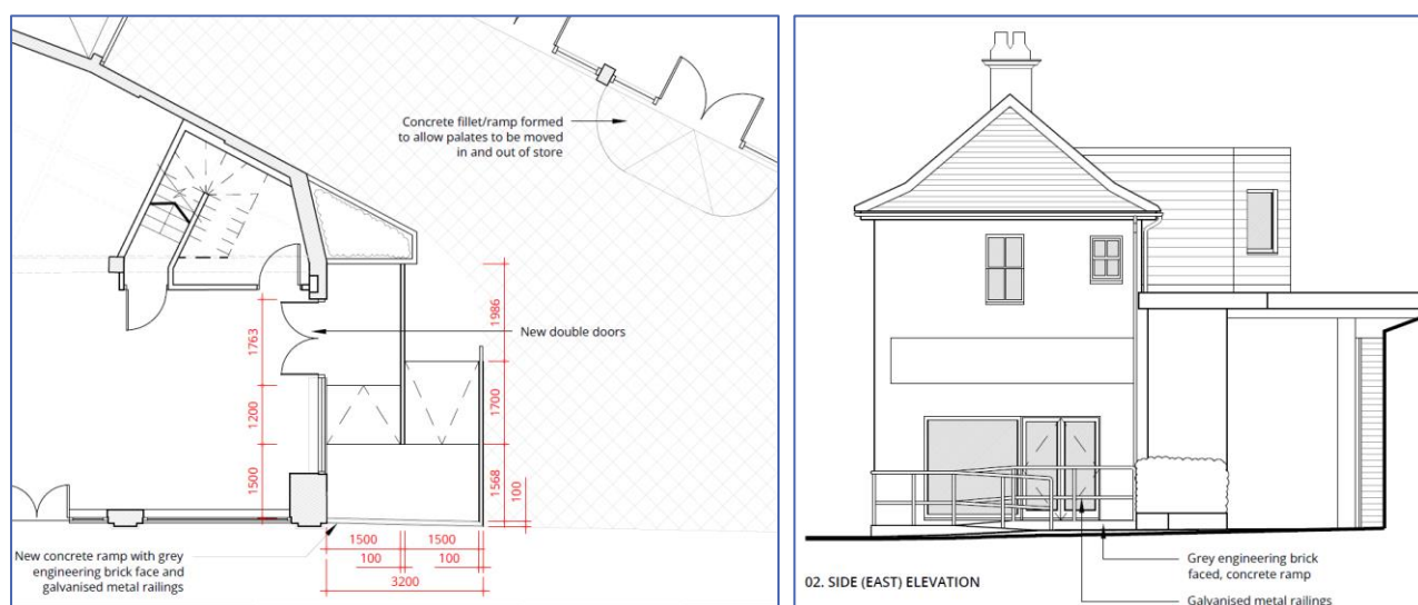
Figures 2 and 3. Extract from Proposed Plan showing the proposed footprint of the ramps and elevation details of the proposed double doors to Unit 1.
