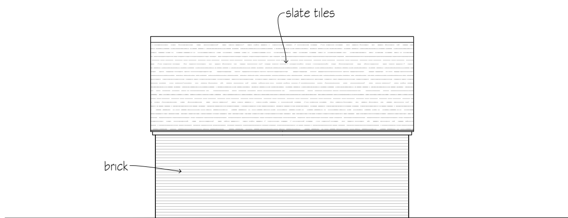
WEST ELEVATION (garage) 1:100
