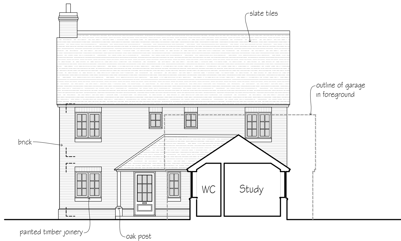
WEST ELEVATION (sectional) 1:100
