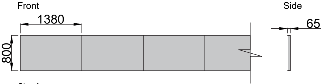
Sign A: ACM-1 Back Panels Size 2 - Ref. 4.52 - 19,190 mm approx. Material: Silver ACM Silver RAL9006, PMS Cool Grey 4 Scale 1:50 @ A3
