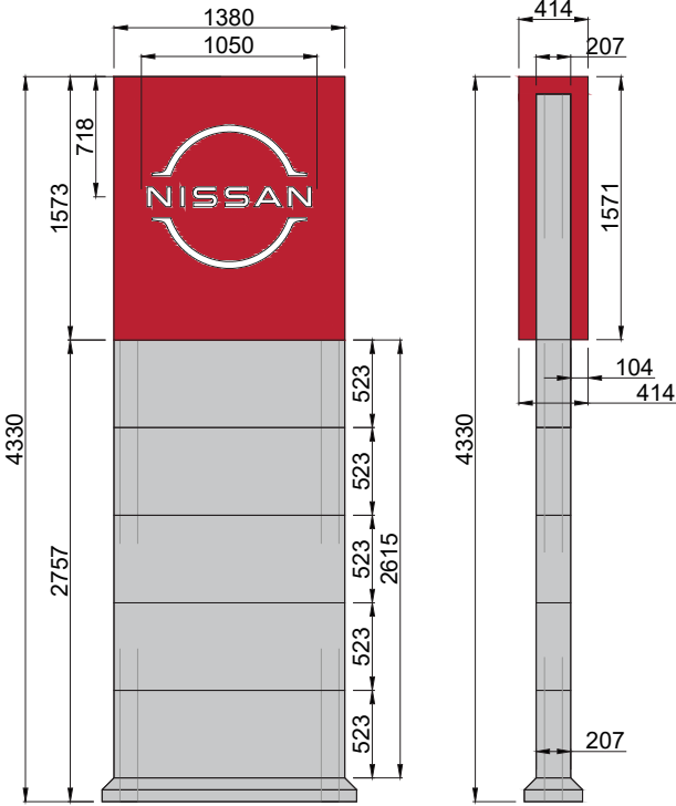
Sign G: Pylon Size 2 Logo Illumination: Internally Illuminated with White LEDs Material: Internal Steel Frame 4mm ACM - Nissan Red NVR-01, RAL3001, PMS200 4mm ACM - Silver - RAL9006, PMS Cool Grey 4 Scale 1:50 @ A3
