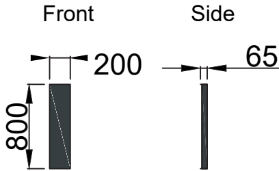
Sign B1, B2: ACM-1 Back Panels Size 2 - Ref. 4.52 Material: ACM Anthracite grey Scale 1:50 @ A3
