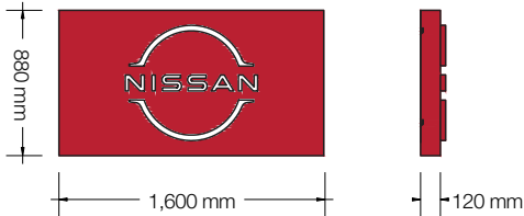
Sign E - Boutique Red Tablet - Size 2 Logo Illumination: Internally Illuminated with White LEDs Material: Internal Aluminium Frame 4mm ACM - Nissan Red NVR-01, RAL3001, PMS200 Scale: 1:50 @ A3
