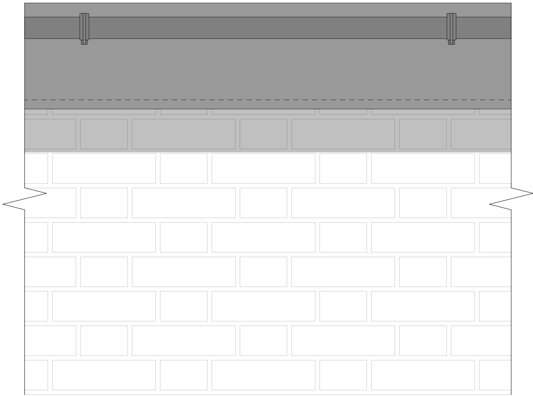
E Flat Roof Verge Elevation Detail Scale: 1:5
