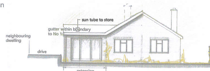
North Elevation
