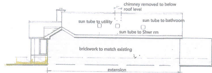
East Elevation
