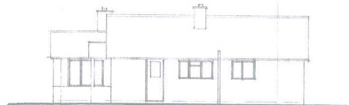
East Elevation
