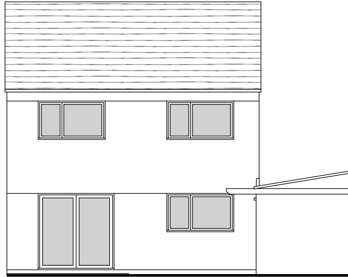
SOUTH ELEVATION
