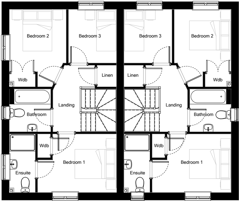
First Floor Plan Plots 9 & 10
