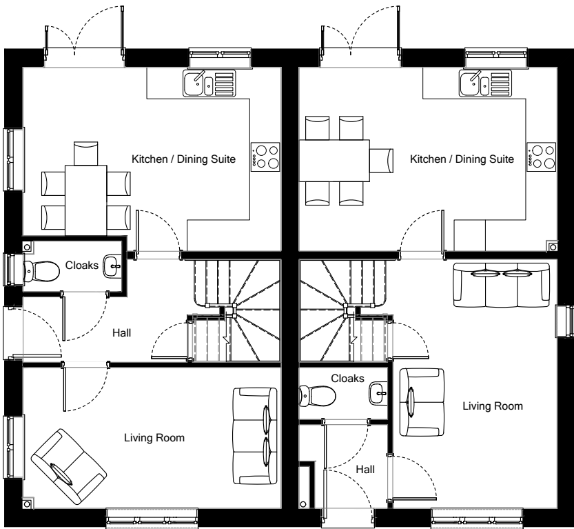
Ground Floor Plan Plots 9 & 10
