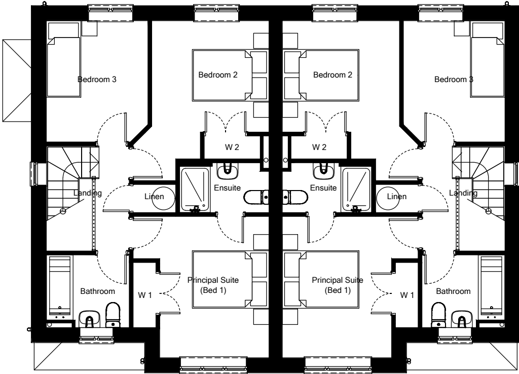
House Type M+ & M - First Floor Plan
