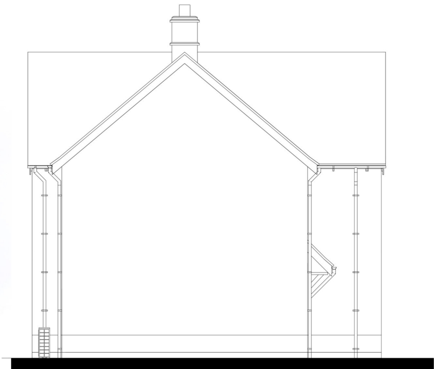
Side Elevation - House Type K
