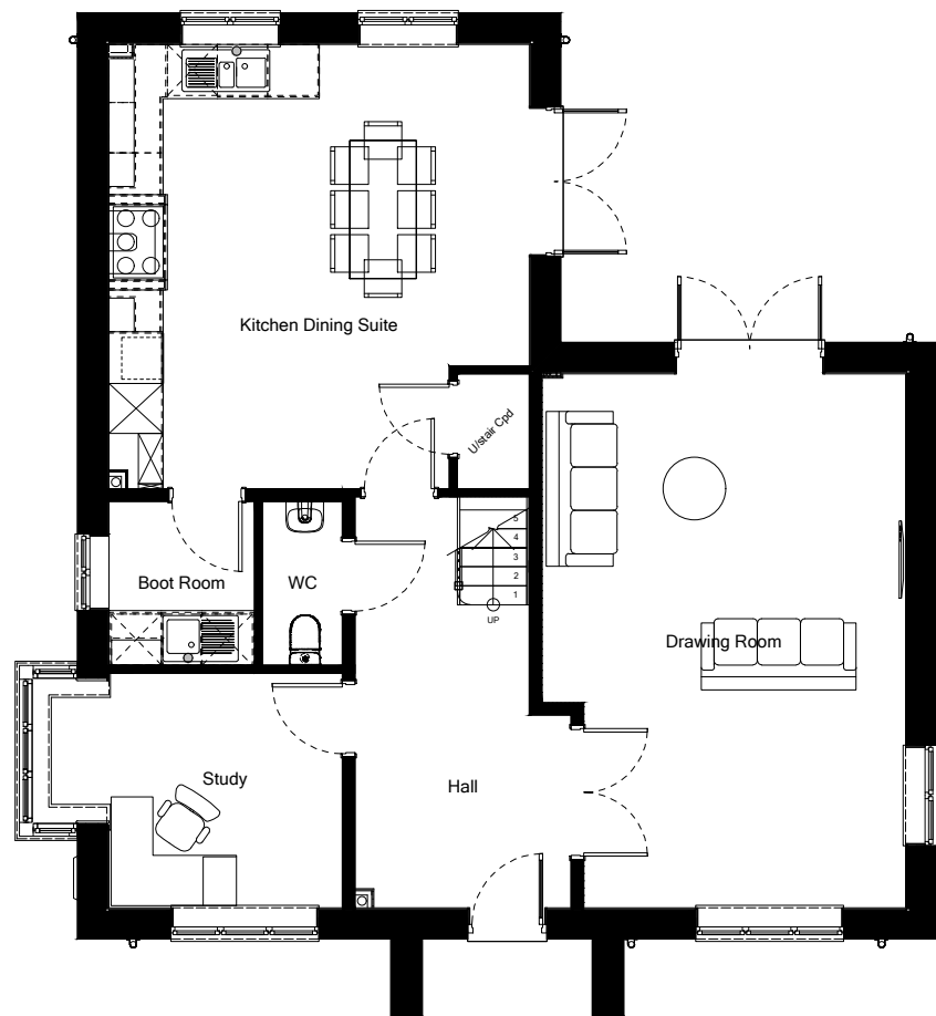
House Type F+ - Ground Floor Plan
